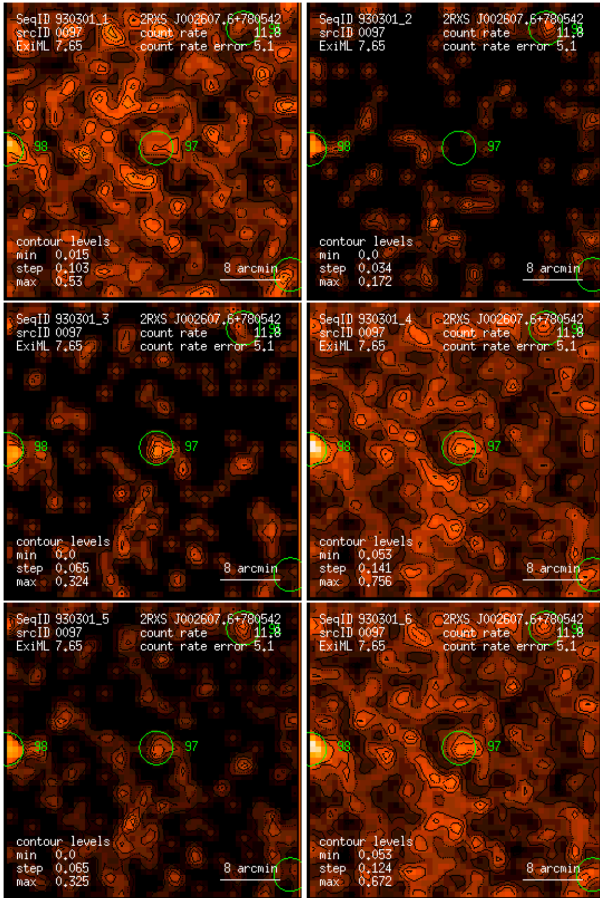
Figure 97: RASS 930301: detection 0097: band rate images, Gaussian filter: (1) PSPC channels 11 – 41, (2) 52 – 90, (3) 91 – 201, (4) 11 – 235, (5) 52 – 201, (6) 11 – 201. Broad band rates in counts/ks. Band rate contour levels in counts/ks/arcmin 2 .
