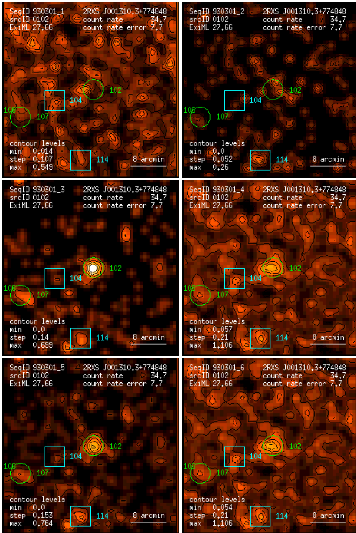
Figure 102: RASS 930301: detection 0102: band rate images, Gaussian filter: (1) PSPC channels 11 – 41, (2) 52 – 90, (3) 91 – 201, (4) 11 – 235, (5) 52 – 201, (6) 11 – 201. Broad band rates in counts/ks. Band rate contour levels in counts/ks/arcmin 2 .
