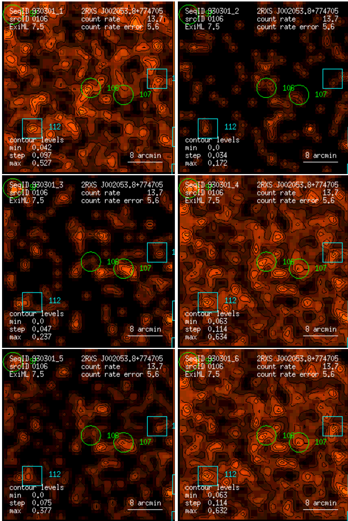
Figure 106: RASS 930301: detection 0106: band rate images, Gaussian filter: (1) PSPC channels 11 – 41, (2) 52 – 90, (3) 91 – 201, (4) 11 – 235, (5) 52 – 201, (6) 11 – 201. Broad band rates in counts/ks. Band rate contour levels in counts/ks/arcmin 2 .
