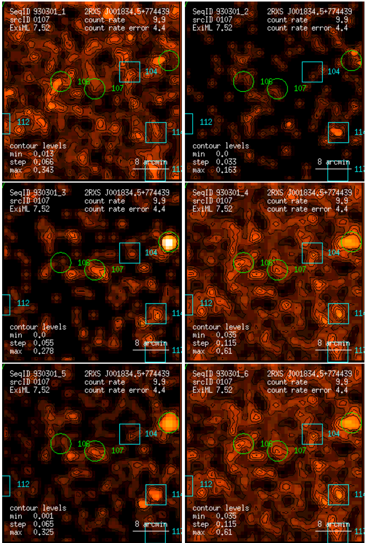
Figure 107: RASS 930301: detection 0107: band rate images, Gaussian filter: (1) PSPC channels 11 – 41, (2) 52 – 90, (3) 91 – 201, (4) 11 – 235, (5) 52 – 201, (6) 11 – 201. Broad band rates in counts/ks. Band rate contour levels in counts/ks/arcmin 2 .
