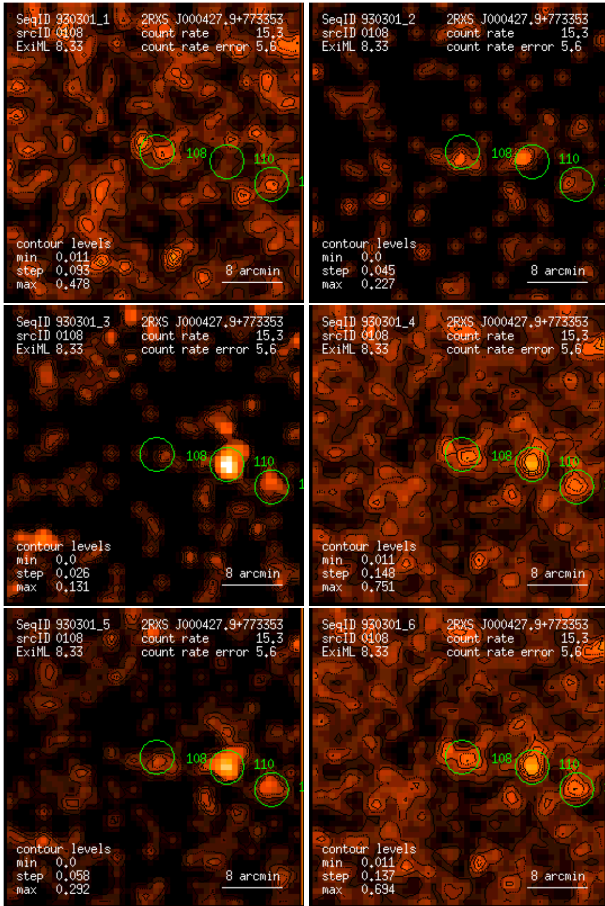
Figure 108: RASS 930301: detection 0108: band rate images, Gaussian filter: (1) PSPC channels 11 – 41, (2) 52 – 90, (3) 91 – 201, (4) 11 – 235, (5) 52 – 201, (6) 11 – 201. Broad band rates in counts/ks. Band rate contour levels in counts/ks/arcmin 2 .
