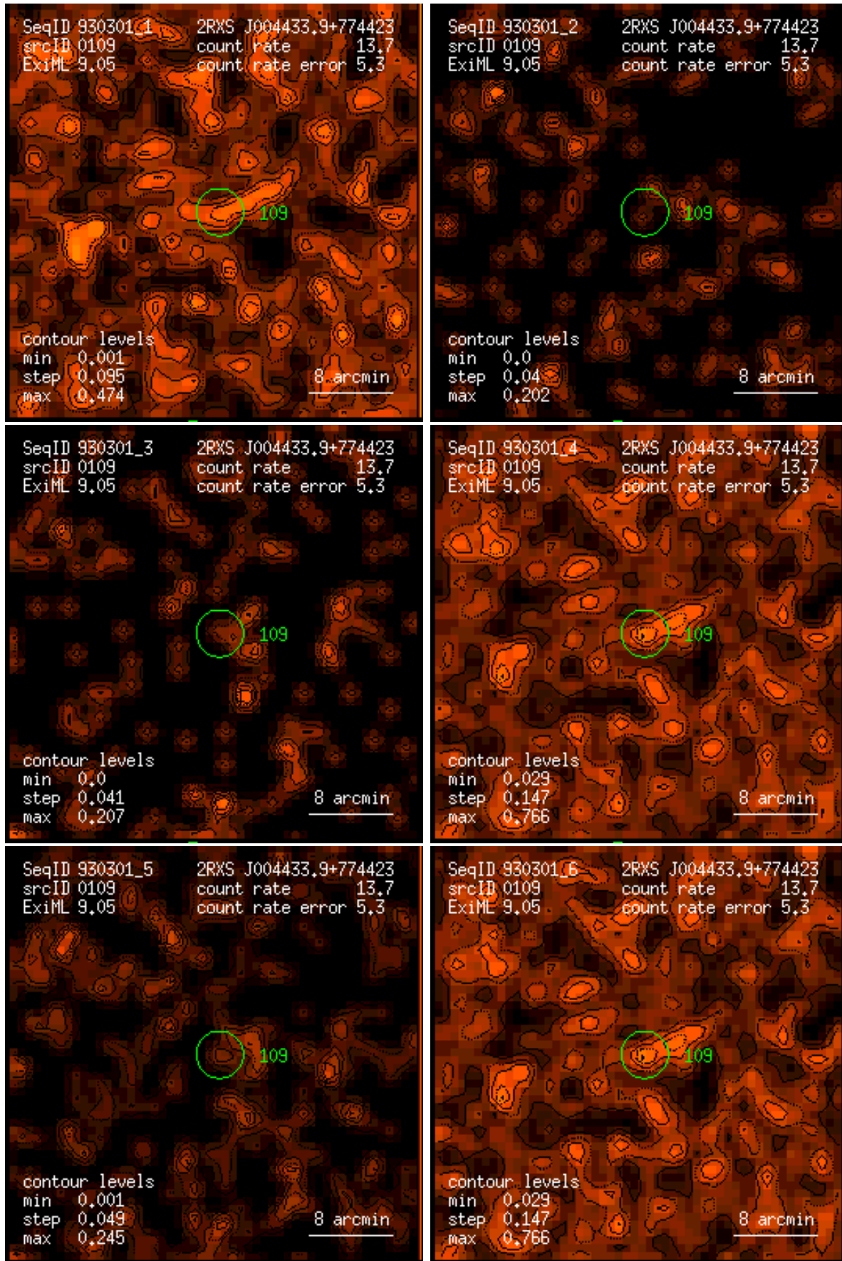
Figure 109: RASS 930301: detection 0109: band rate images, Gaussian filter: (1) PSPC channels 11 – 41, (2) 52 – 90, (3) 91 – 201, (4) 11 – 235, (5) 52 – 201, (6) 11 – 201. Broad band rates in counts/ks. Band rate contour levels in counts/ks/arcmin 2 .
