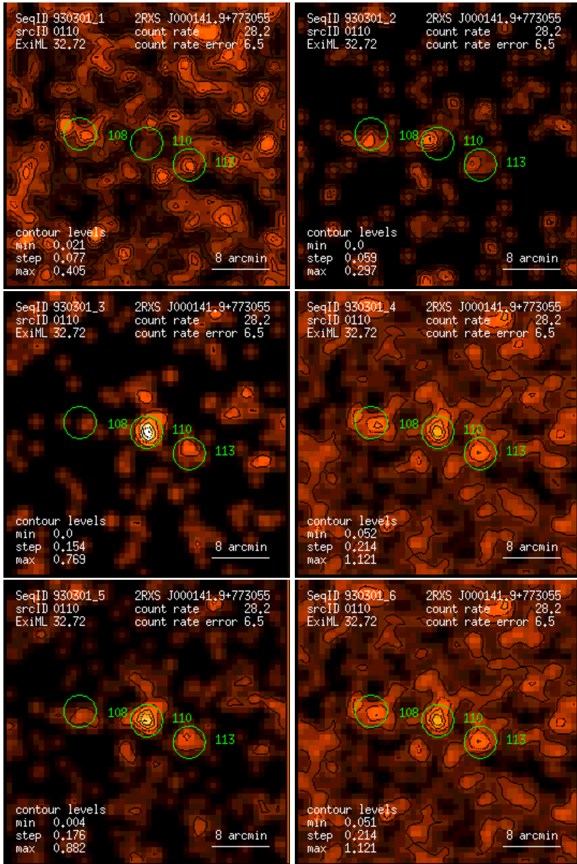
Figure 110: RASS 930301: detection 0110: band rate images, Gaussian filter: (1) PSPC channels 11 – 41, (2) 52 – 90, (3) 91 – 201, (4) 11 – 235, (5) 52 – 201, (6) 11 – 201. Broad band rates in counts/ks. Band rate contour levels in counts/ks/arcmin 2 .
