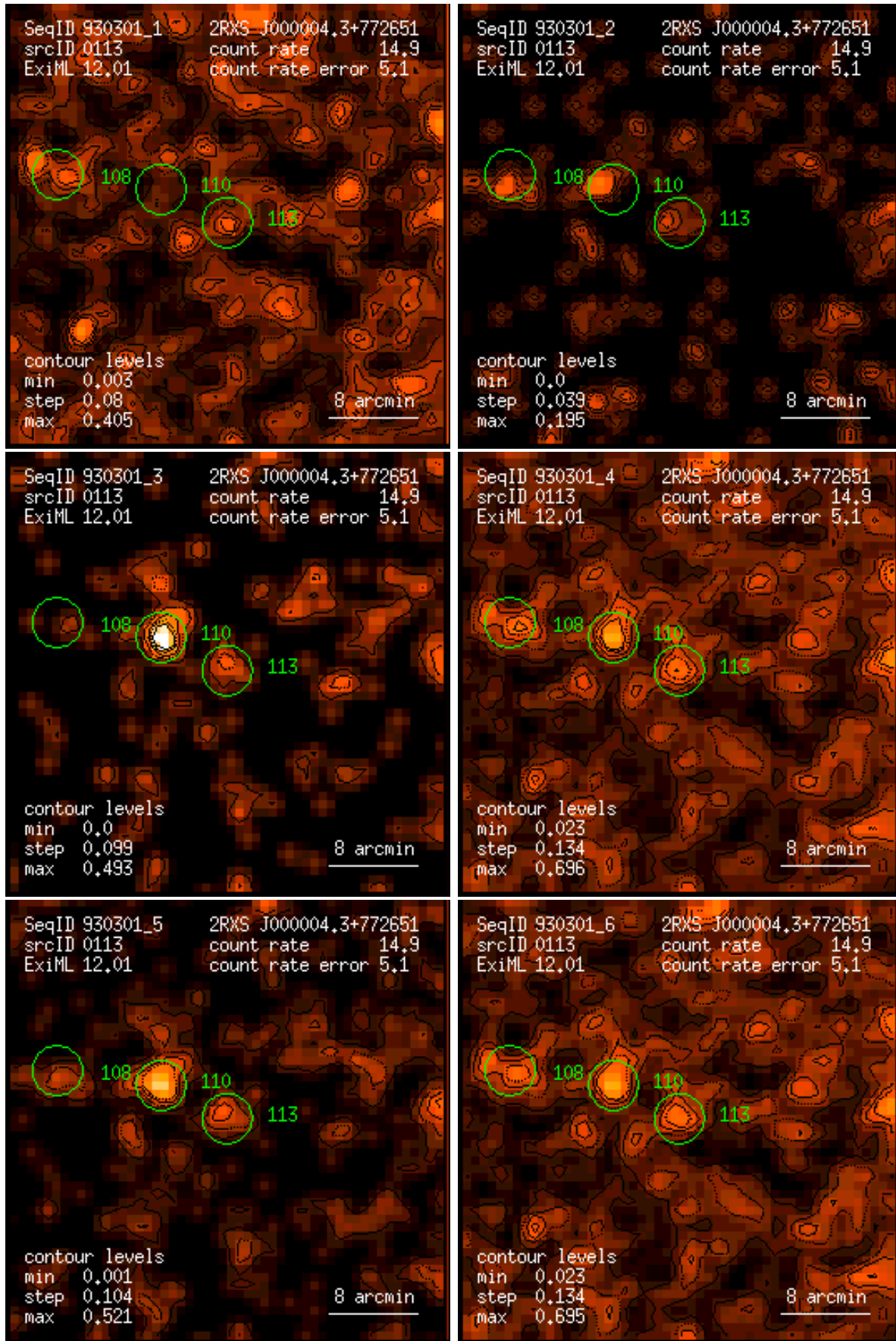
Figure 113: RASS 930301: detection 0113: band rate images, Gaussian filter: (1) PSPC channels 11 – 41, (2) 52 – 90, (3) 91 – 201, (4) 11 – 235, (5) 52 – 201, (6) 11 – 201. Broad band rates in counts/ks. Band rate contour levels in counts/ks/arcmin 2 .
