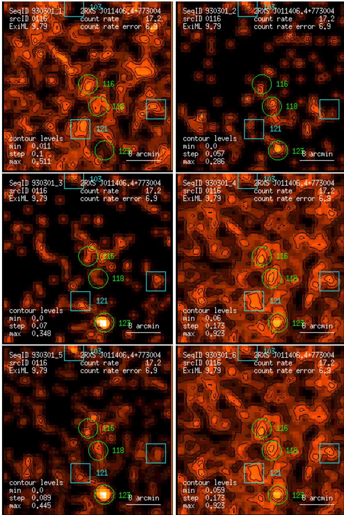
Figure 116: RASS 930301: detection 0116: band rate images, Gaussian filter: (1) PSPC channels 11 – 41, (2) 52 – 90, (3) 91 – 201, (4) 11 – 235, (5) 52 – 201, (6) 11 – 201. Broad band rates in counts/ks. Band rate contour levels in counts/ks/arcmin 2 .
