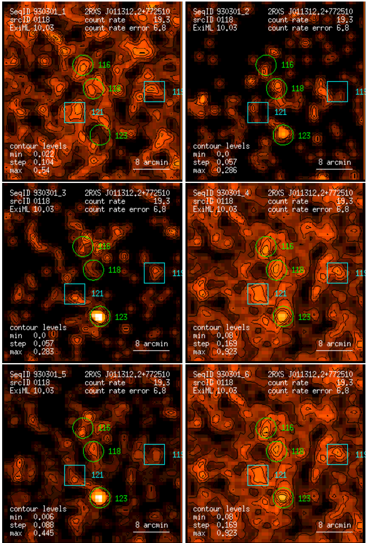
Figure 118: RASS 930301: detection 0118: band rate images, Gaussian filter: (1) PSPC channels 11 – 41, (2) 52 – 90, (3) 91 – 201, (4) 11 – 235, (5) 52 – 201, (6) 11 – 201. Broad band rates in counts/ks. Band rate contour levels in counts/ks/arcmin 2 .
