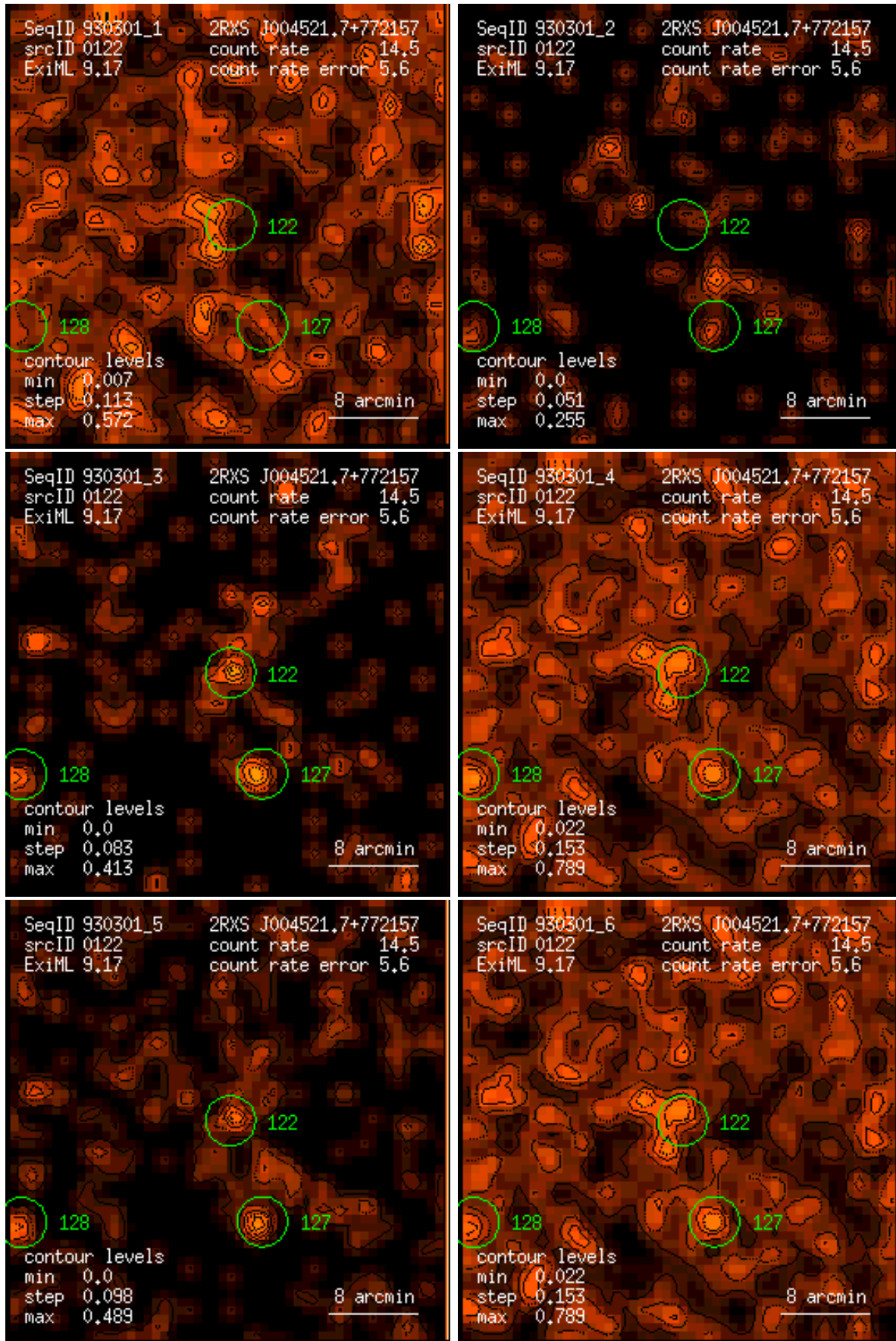
Figure 122: RASS 930301: detection 0122: band rate images, Gaussian filter: (1) PSPC channels 11 – 41, (2) 52 – 90, (3) 91 – 201, (4) 11 – 235, (5) 52 – 201, (6) 11 – 201. Broad band rates in counts/ks. Band rate contour levels in counts/ks/arcmin 2 .
