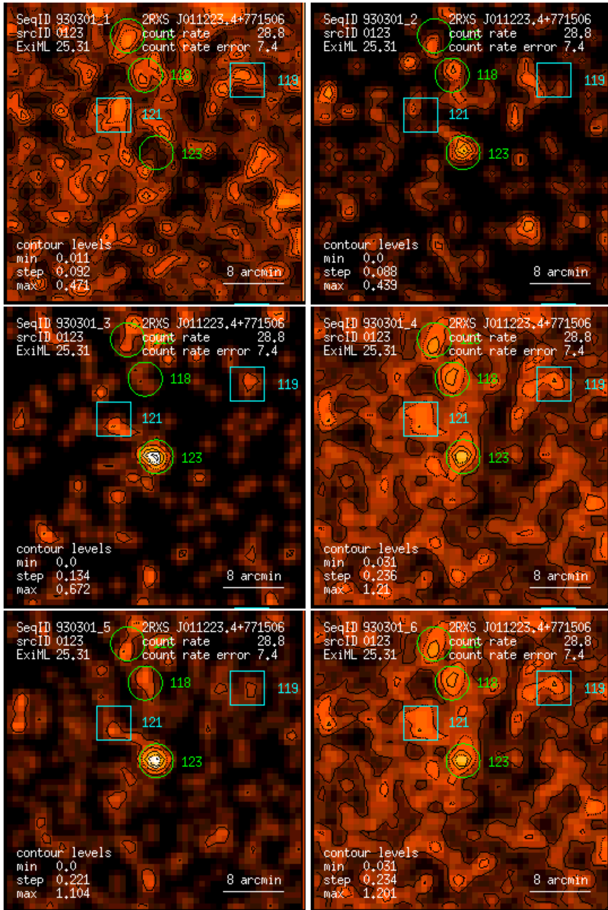
Figure 123: RASS 930301: detection 0123: band rate images, Gaussian filter: (1) PSPC channels 11 – 41, (2) 52 – 90, (3) 91 – 201, (4) 11 – 235, (5) 52 – 201, (6) 11 – 201. Broad band rates in counts/ks. Band rate contour levels in counts/ks/arcmin 2 .
