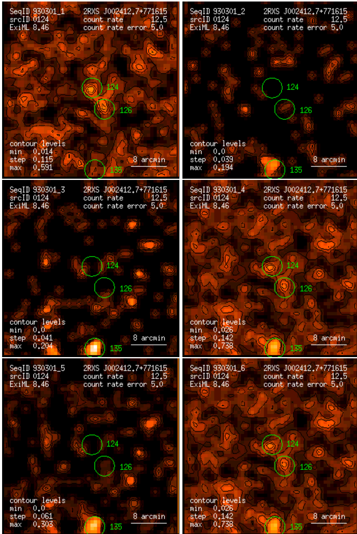
Figure 124: RASS 930301: detection 0124: band rate images, Gaussian filter: (1) PSPC channels 11 – 41, (2) 52 – 90, (3) 91 – 201, (4) 11 – 235, (5) 52 – 201, (6) 11 – 201. Broad band rates in counts/ks. Band rate contour levels in counts/ks/arcmin 2 .
