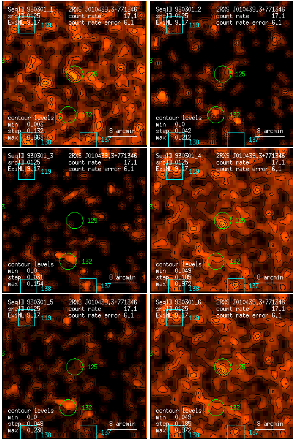
Figure 125: RASS 930301: detection 0125: band rate images, Gaussian filter: (1) PSPC channels 11 – 41, (2) 52 – 90, (3) 91 – 201, (4) 11 – 235, (5) 52 – 201, (6) 11 – 201. Broad band rates in counts/ks. Band rate contour levels in counts/ks/arcmin 2 .
