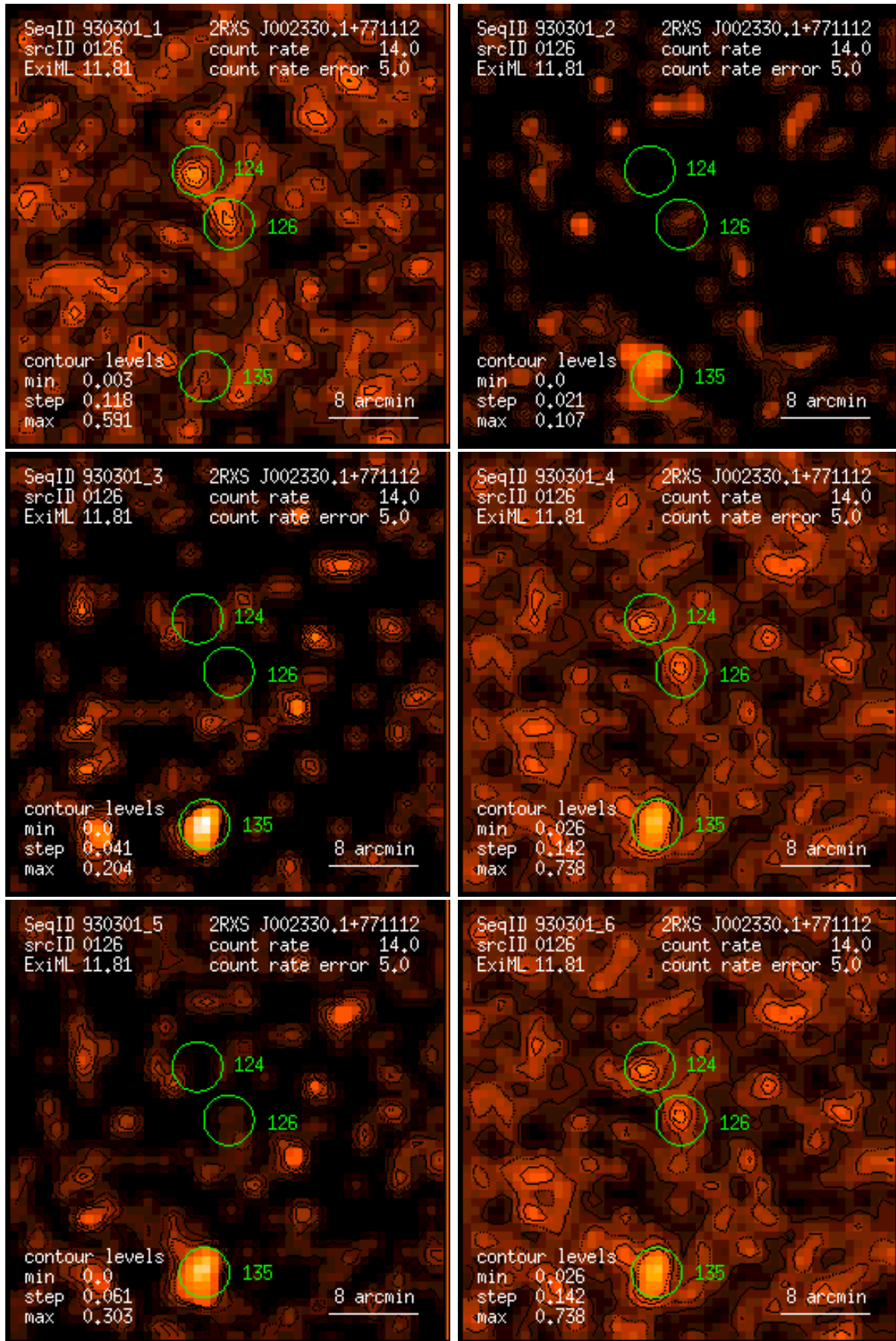
Figure 126: RASS 930301: detection 0126: band rate images, Gaussian filter: (1) PSPC channels 11 – 41, (2) 52 – 90, (3) 91 – 201, (4) 11 – 235, (5) 52 – 201, (6) 11 – 201. Broad band rates in counts/ks. Band rate contour levels in counts/ks/arcmin 2 .
