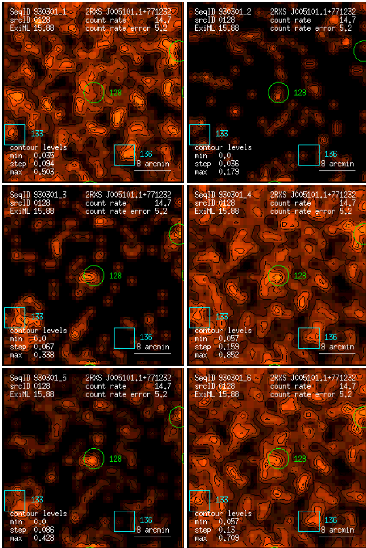
Figure 128: RASS 930301: detection 0128: band rate images, Gaussian filter: (1) PSPC channels 11 – 41, (2) 52 – 90, (3) 91 – 201, (4) 11 – 235, (5) 52 – 201, (6) 11 – 201. Broad band rates in counts/ks. Band rate contour levels in counts/ks/arcmin 2 .
