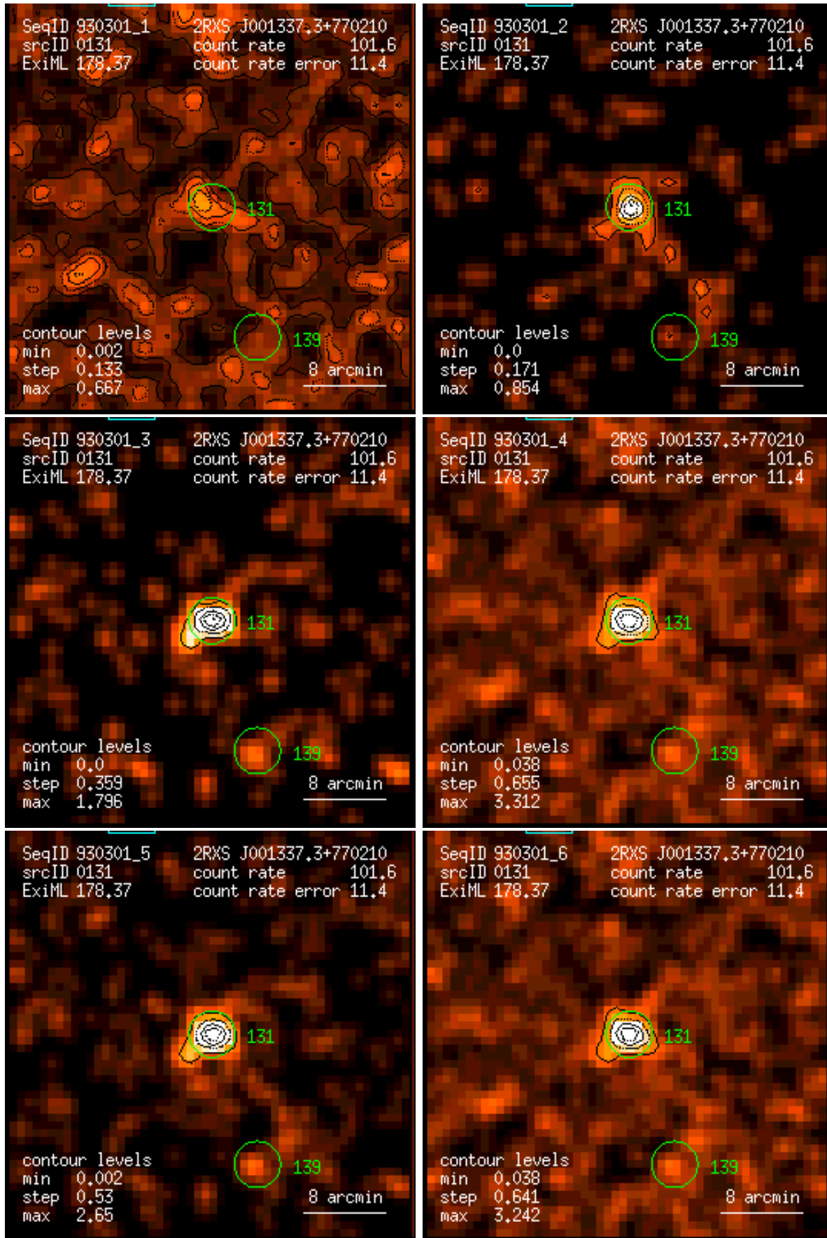
Figure 131: RASS 930301: detection 0131: band rate images, Gaussian filter: (1) PSPC channels 11 – 41, (2) 52 – 90, (3) 91 – 201, (4) 11 – 235, (5) 52 – 201, (6) 11 – 201. Broad band rates in counts/ks. Band rate contour levels in counts/ks/arcmin 2 .
