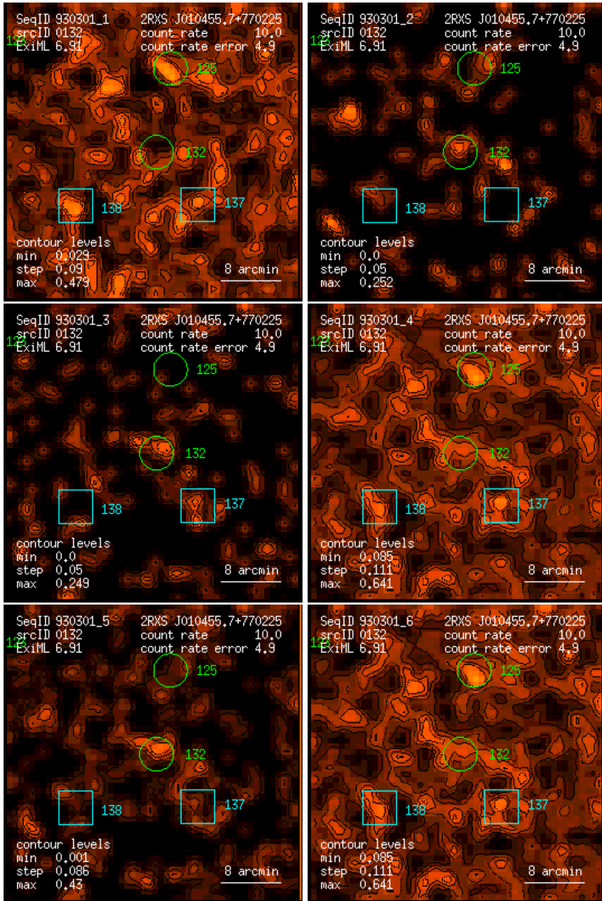
Figure 132: RASS 930301: detection 0132: band rate images, Gaussian filter: (1) PSPC channels 11 – 41, (2) 52 – 90, (3) 91 – 201, (4) 11 – 235, (5) 52 – 201, (6) 11 – 201. Broad band rates in counts/ks. Band rate contour levels in counts/ks/arcmin 2 .
