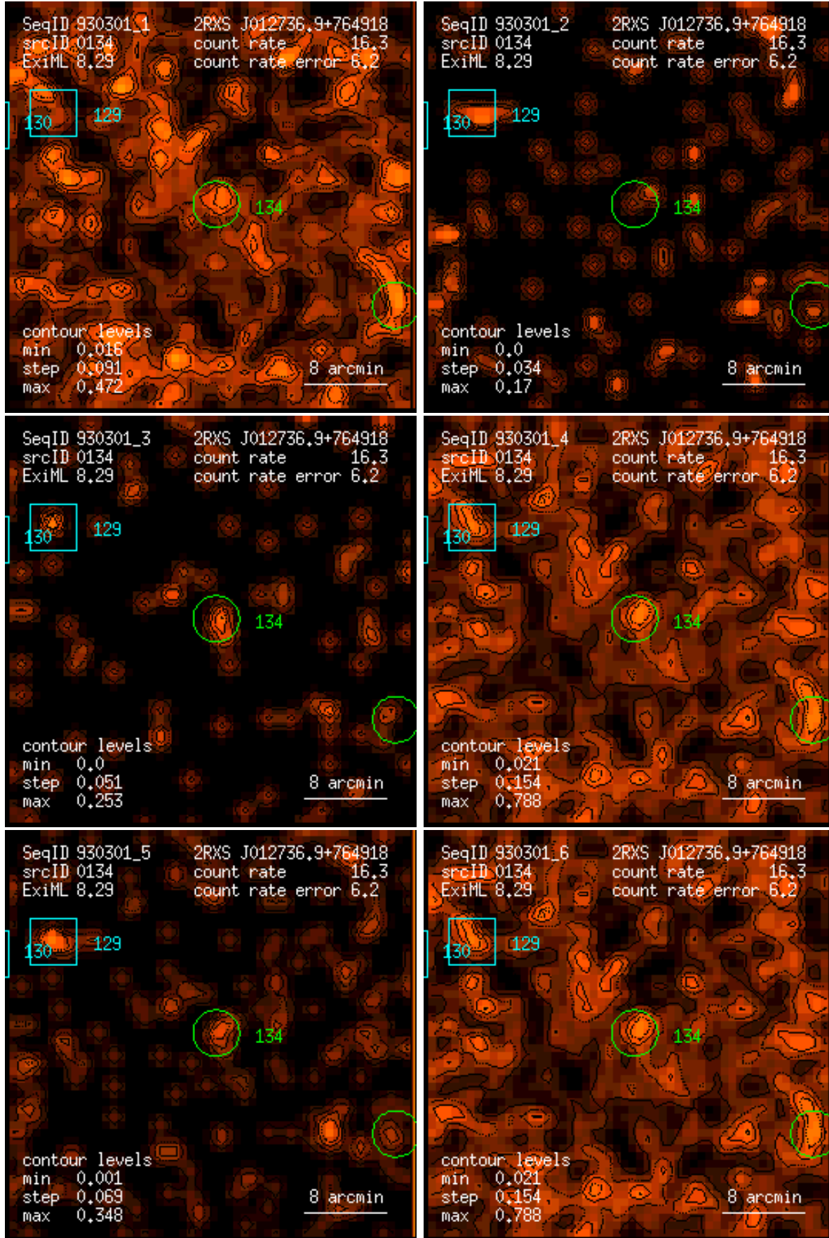
Figure 134: RASS 930301: detection 0134: band rate images, Gaussian filter: (1) PSPC channels 11 – 41, (2) 52 – 90, (3) 91 – 201, (4) 11 – 235, (5) 52 – 201, (6) 11 – 201. Broad band rates in counts/ks. Band rate contour levels in counts/ks/arcmin 2 .
