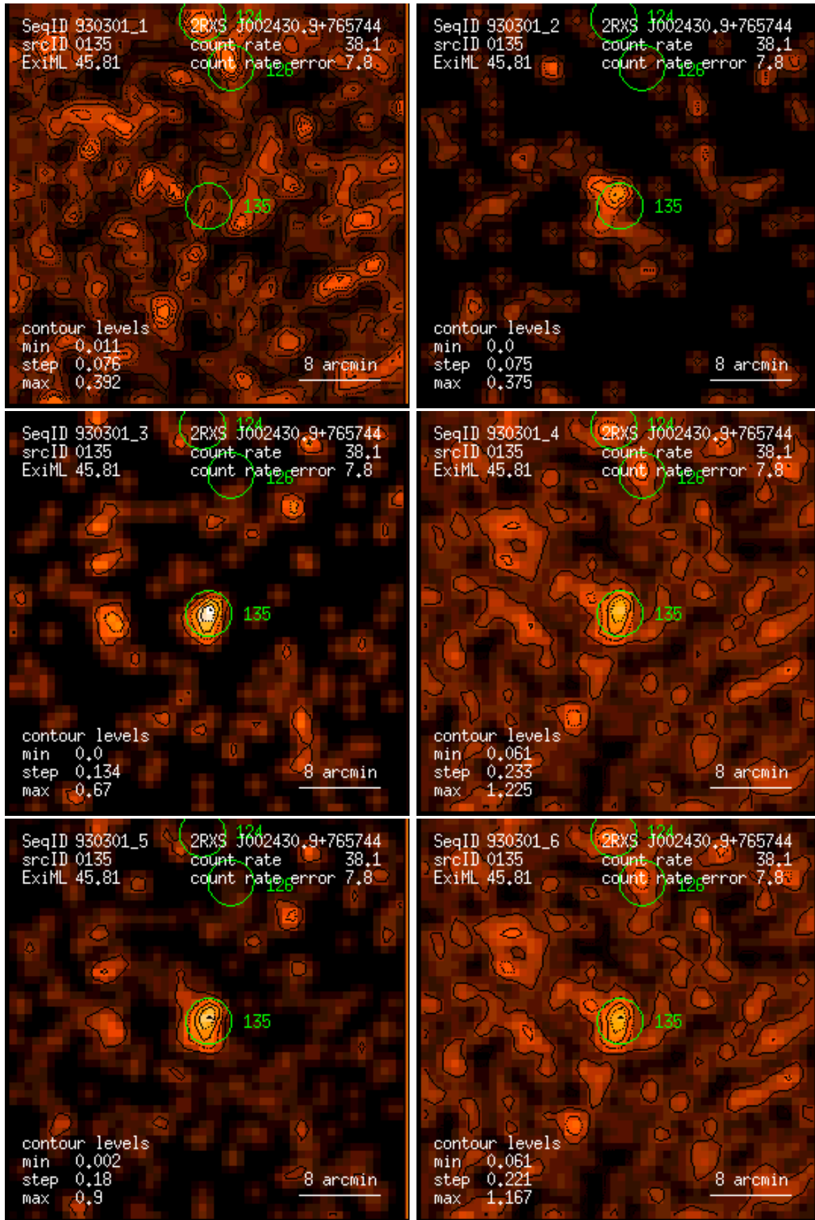
Figure 135: RASS 930301: detection 0135: band rate images, Gaussian filter: (1) PSPC channels 11 – 41, (2) 52 – 90, (3) 91 – 201, (4) 11 – 235, (5) 52 – 201, (6) 11 – 201. Broad band rates in counts/ks. Band rate contour levels in counts/ks/arcmin 2 .
