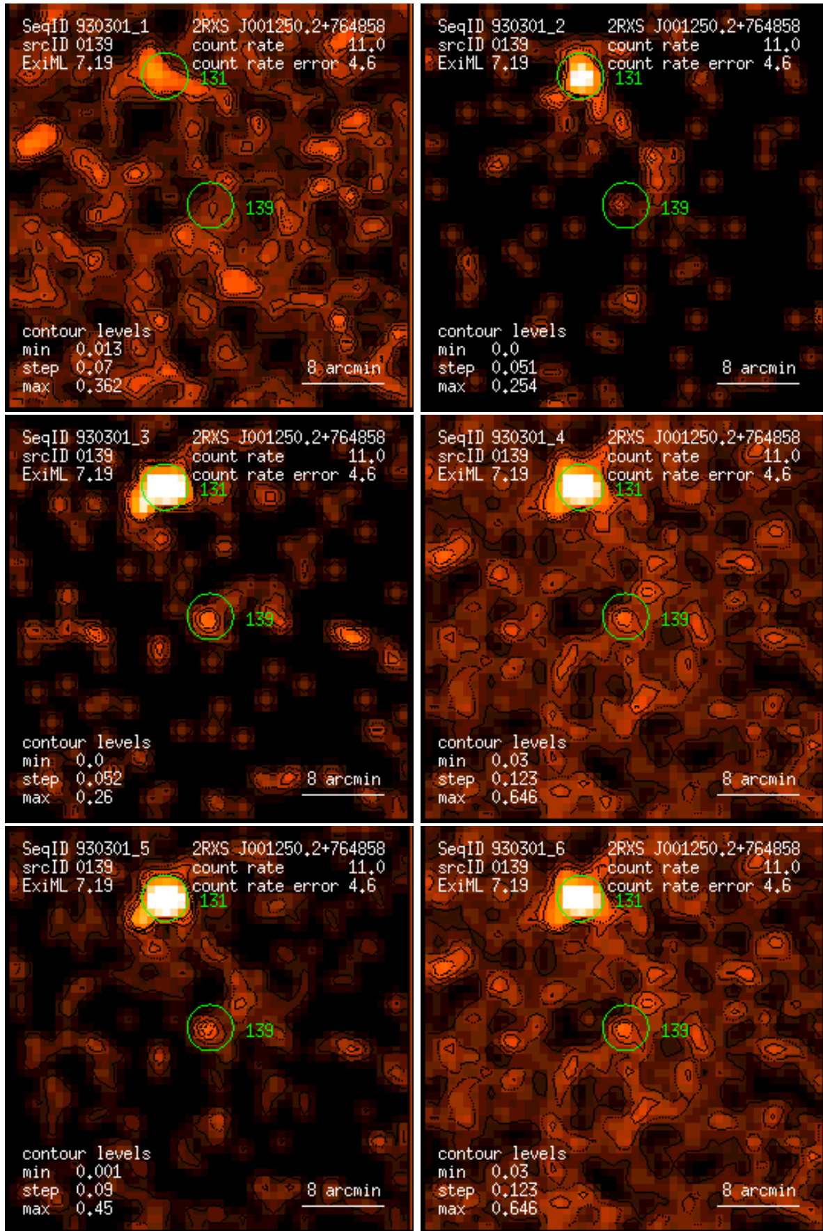
Figure 139: RASS 930301: detection 0139: band rate images, Gaussian filter: (1) PSPC channels 11 – 41, (2) 52 – 90, (3) 91 – 201, (4) 11 – 235, (5) 52 – 201, (6) 11 – 201. Broad band rates in counts/ks. Band rate contour levels in counts/ks/arcmin 2 .
