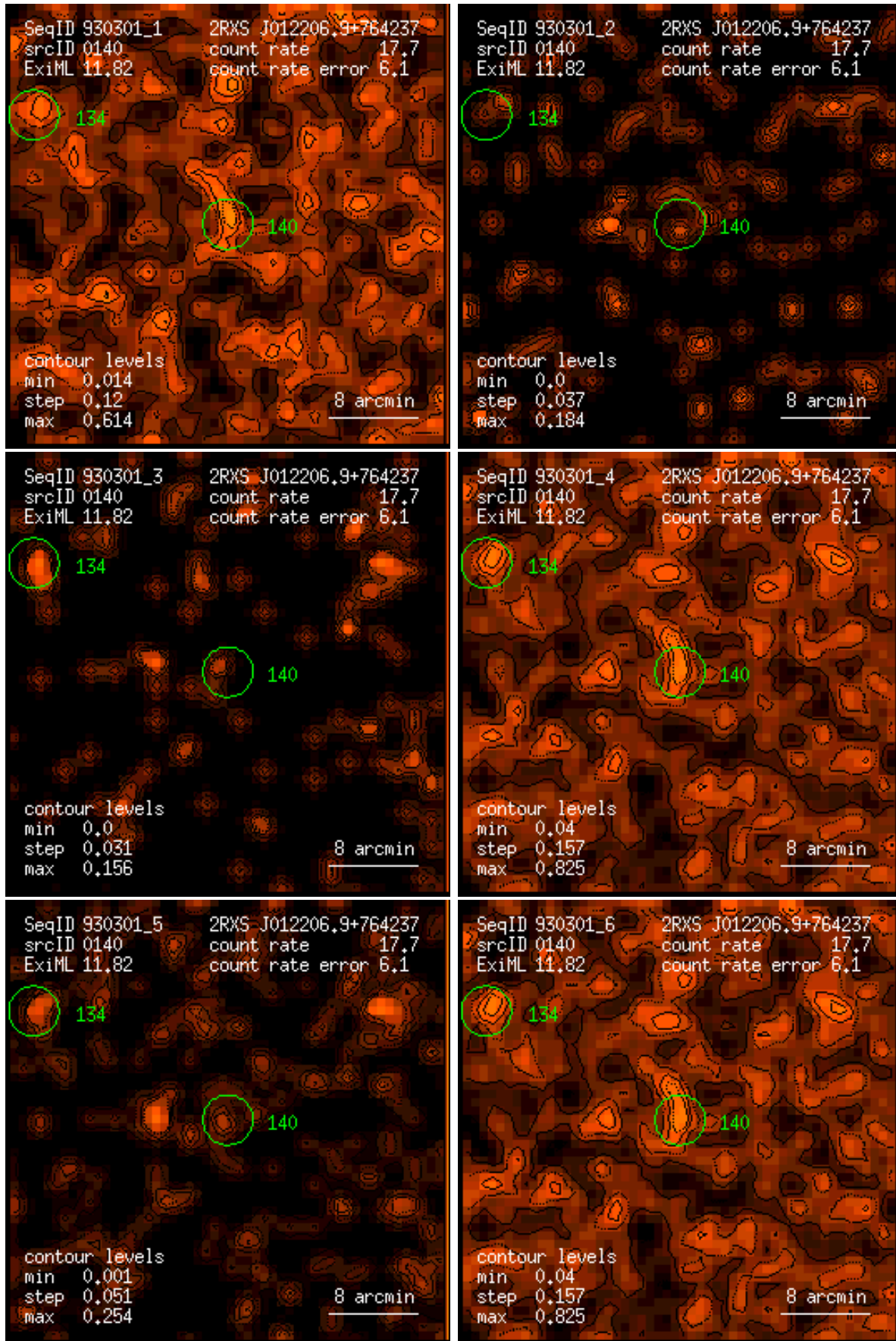
Figure 140: RASS 930301: detection 0140: band rate images, Gaussian filter: (1) PSPC channels 11 – 41, (2) 52 – 90, (3) 91 – 201, (4) 11 – 235, (5) 52 – 201, (6) 11 – 201. Broad band rates in counts/ks. Band rate contour levels in counts/ks/arcmin 2 .
