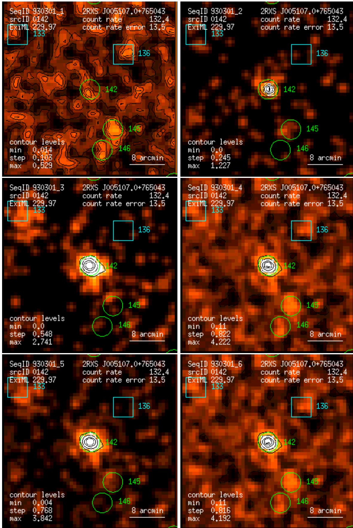
Figure 142: RASS 930301: detection 0142: band rate images, Gaussian filter: (1) PSPC channels 11 – 41, (2) 52 – 90, (3) 91 – 201, (4) 11 – 235, (5) 52 – 201, (6) 11 – 201. Broad band rates in counts/ks. Band rate contour levels in counts/ks/arcmin 2 .
