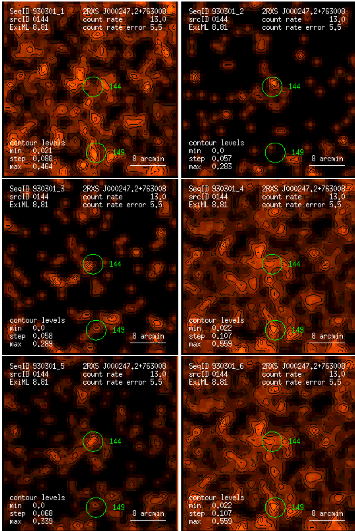
Figure 144: RASS 930301: detection 0144: band rate images, Gaussian filter: (1) PSPC channels 11 – 41, (2) 52 – 90, (3) 91 – 201, (4) 11 – 235, (5) 52 – 201, (6) 11 – 201. Broad band rates in counts/ks. Band rate contour levels in counts/ks/arcmin 2 .
