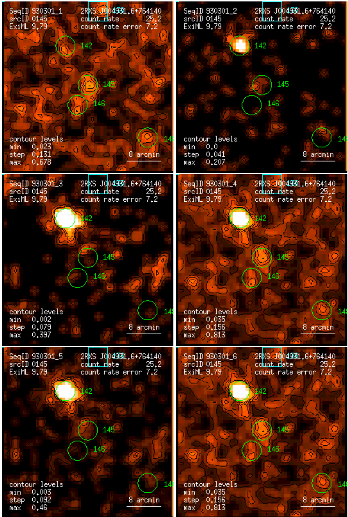
Figure 145: RASS 930301: detection 0145: band rate images, Gaussian filter: (1) PSPC channels 11 – 41, (2) 52 – 90, (3) 91 – 201, (4) 11 – 235, (5) 52 – 201, (6) 11 – 201. Broad band rates in counts/ks. Band rate contour levels in counts/ks/arcmin 2 .
