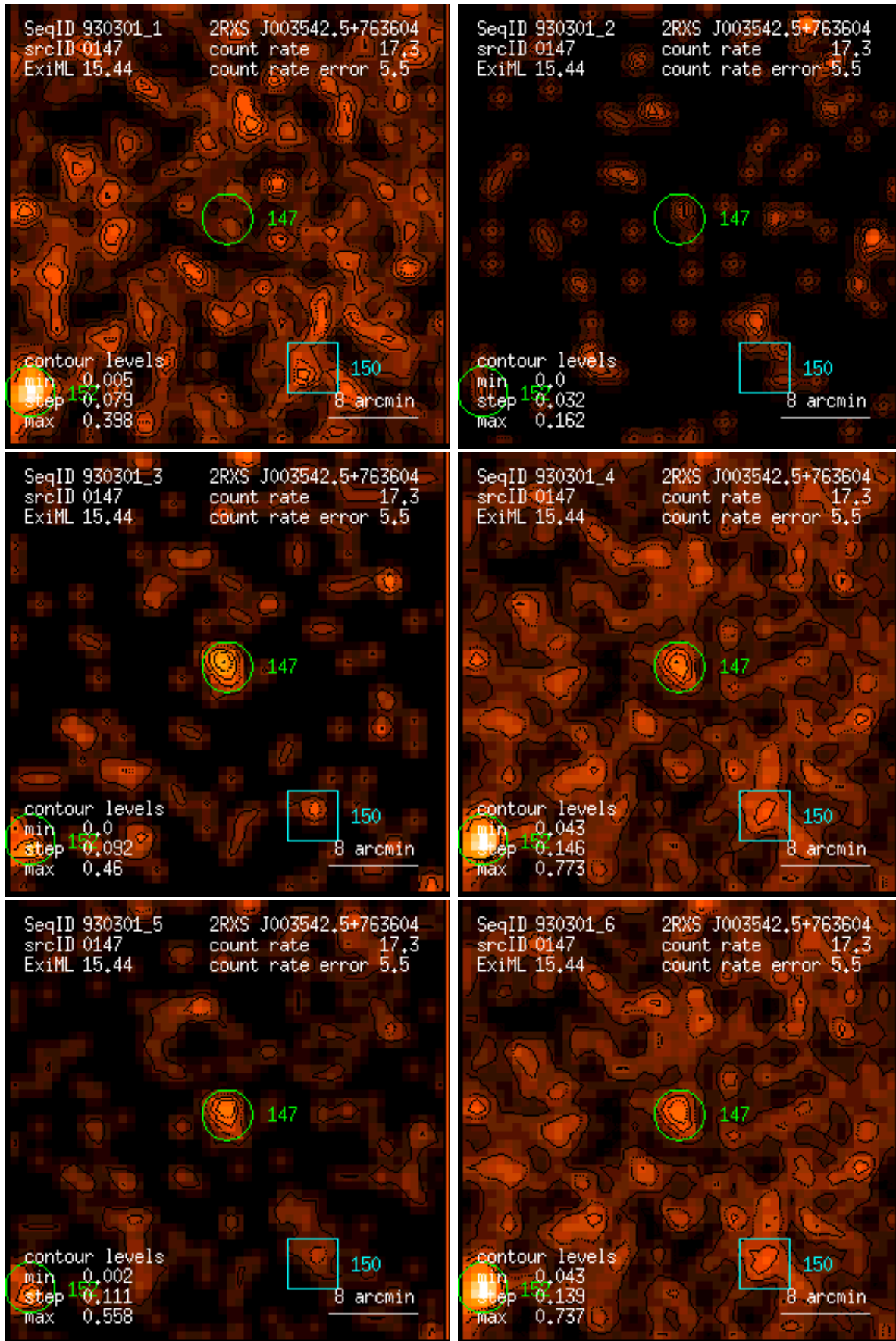
Figure 147: RASS 930301: detection 0147: band rate images, Gaussian filter: (1) PSPC channels 11 – 41, (2) 52 – 90, (3) 91 – 201, (4) 11 – 235, (5) 52 – 201, (6) 11 – 201. Broad band rates in counts/ks. Band rate contour levels in counts/ks/arcmin 2 .
