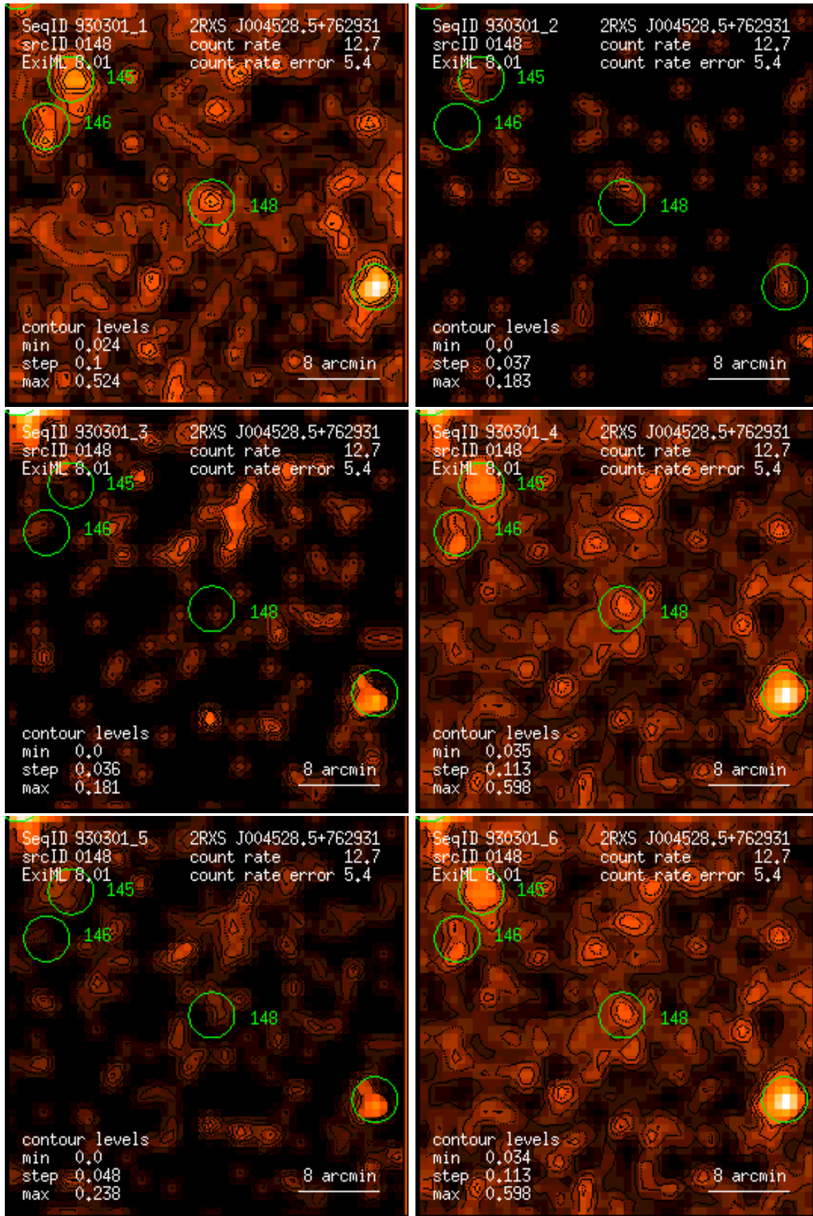
Figure 148: RASS 930301: detection 0148: band rate images, Gaussian filter: (1) PSPC channels 11 – 41, (2) 52 – 90, (3) 91 – 201, (4) 11 – 235, (5) 52 – 201, (6) 11 – 201. Broad band rates in counts/ks. Band rate contour levels in counts/ks/arcmin 2 .
