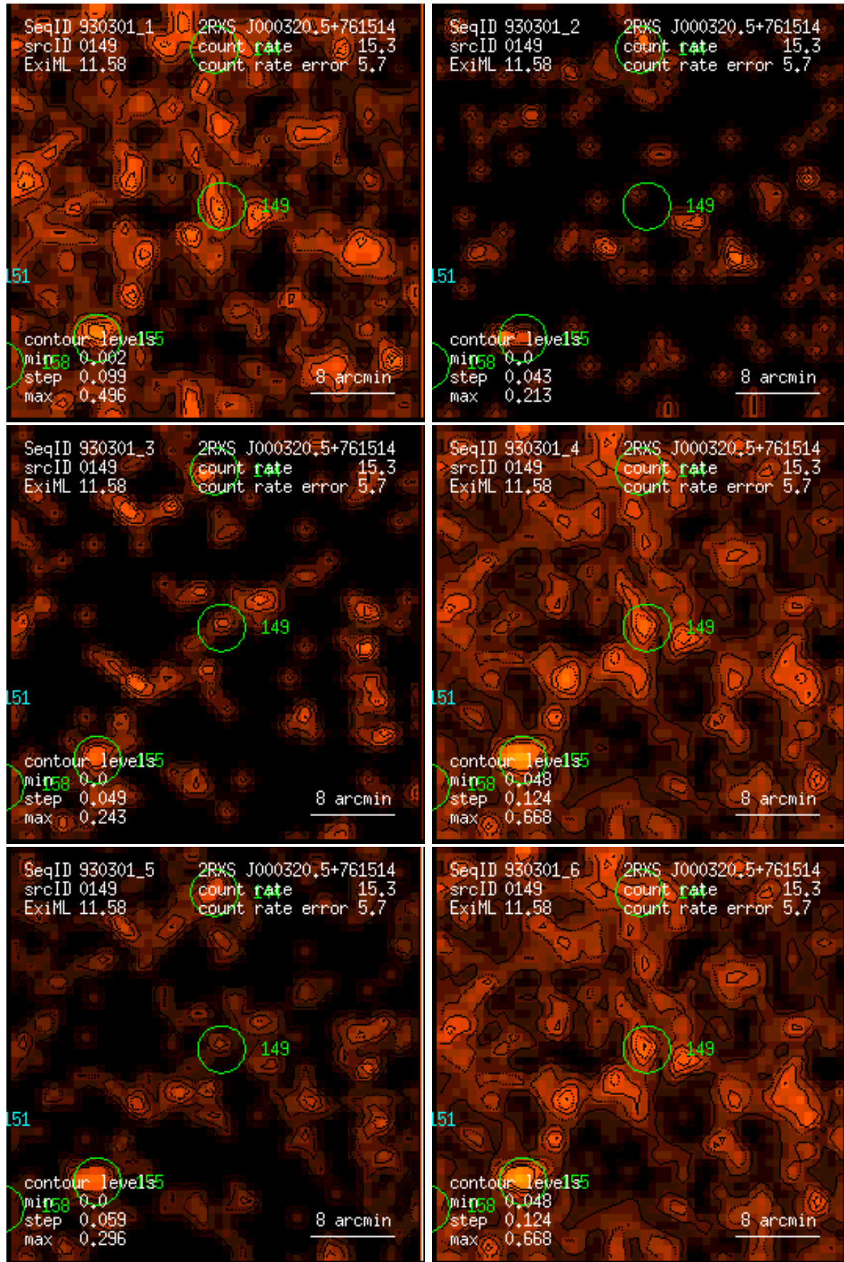
Figure 149: RASS 930301: detection 0149: band rate images, Gaussian filter: (1) PSPC channels 11 – 41, (2) 52 – 90, (3) 91 – 201, (4) 11 – 235, (5) 52 – 201, (6) 11 – 201. Broad band rates in counts/ks. Band rate contour levels in counts/ks/arcmin 2 .
