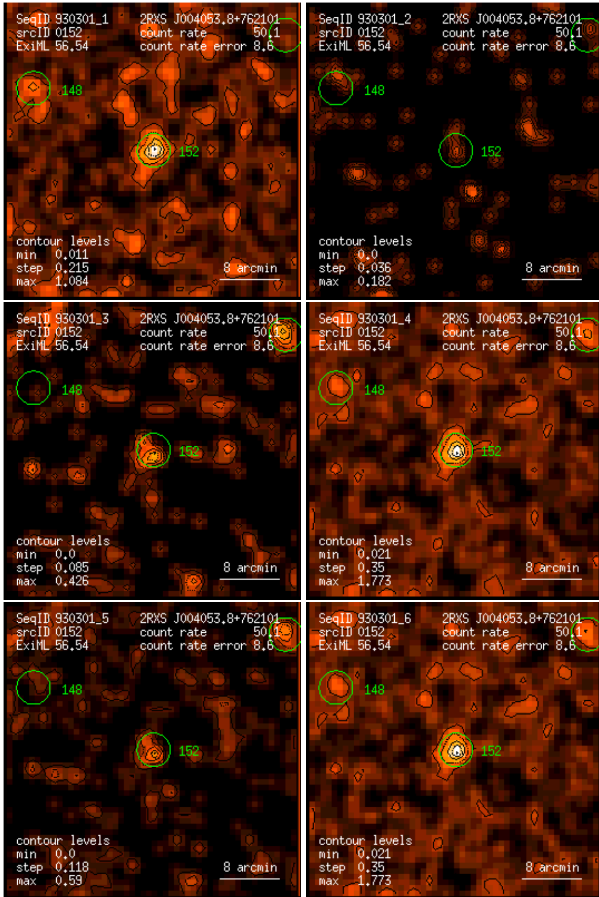
Figure 152: RASS 930301: detection 0152: band rate images, Gaussian filter: (1) PSPC channels 11 – 41, (2) 52 – 90, (3) 91 – 201, (4) 11 – 235, (5) 52 – 201, (6) 11 – 201. Broad band rates in counts/ks. Band rate contour levels in counts/ks/arcmin 2 .
