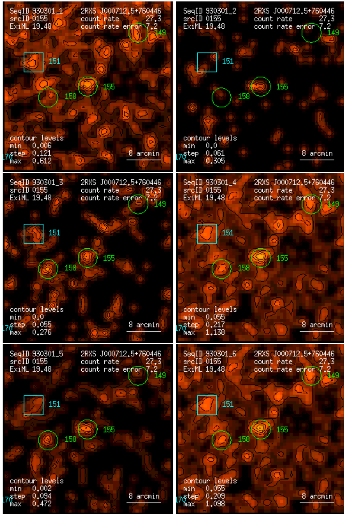
Figure 155: RASS 930301: detection 0155: band rate images, Gaussian filter: (1) PSPC channels 11 – 41, (2) 52 – 90, (3) 91 – 201, (4) 11 – 235, (5) 52 – 201, (6) 11 – 201. Broad band rates in counts/ks. Band rate contour levels in counts/ks/arcmin 2 .
