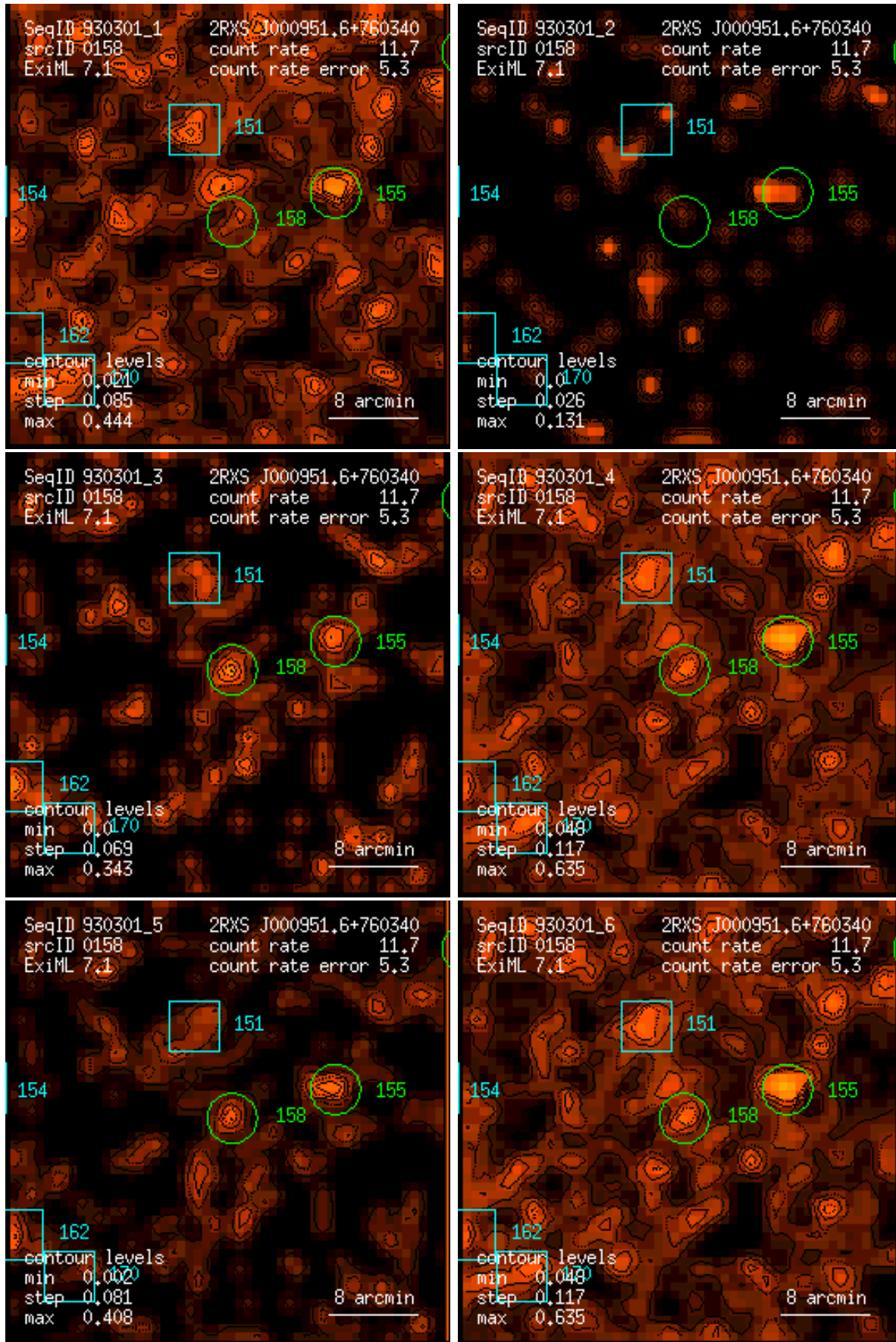
Figure 158: RASS 930301: detection 0158: band rate images, Gaussian filter: (1) PSPC channels 11 – 41, (2) 52 – 90, (3) 91 – 201, (4) 11 – 235, (5) 52 – 201, (6) 11 – 201. Broad band rates in counts/ks. Band rate contour levels in counts/ks/arcmin 2 .
