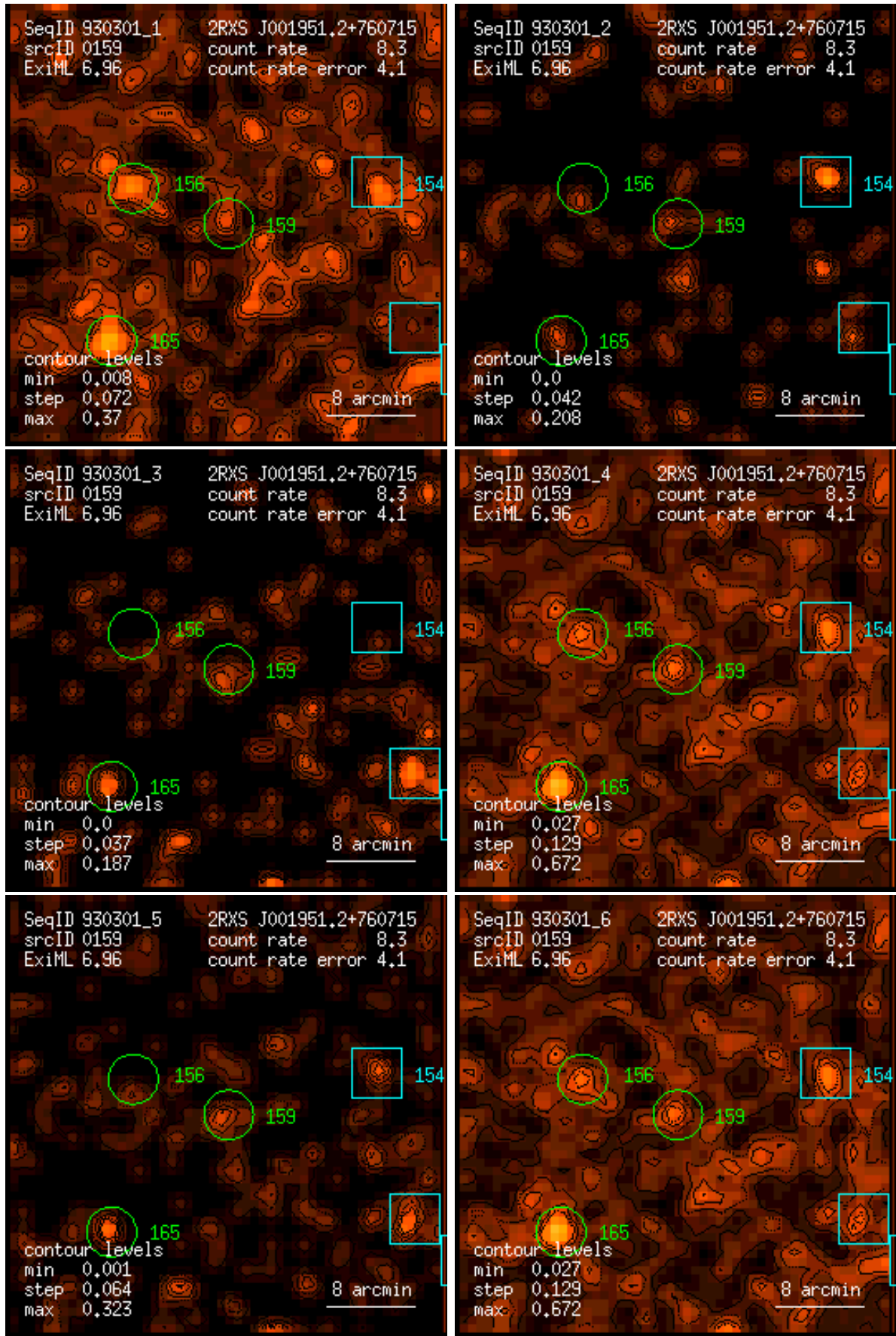
Figure 159: RASS 930301: detection 0159: band rate images, Gaussian filter: (1) PSPC channels 11 – 41, (2) 52 – 90, (3) 91 – 201, (4) 11 – 235, (5) 52 – 201, (6) 11 – 201. Broad band rates in counts/ks. Band rate contour levels in counts/ks/arcmin 2 .
