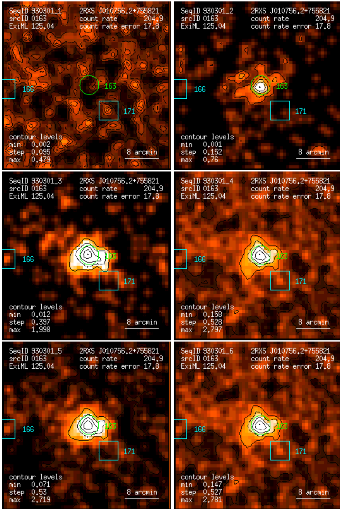
Figure 163: RASS 930301: detection 0163: band rate images, Gaussian filter: (1) PSPC channels 11 – 41, (2) 52 – 90, (3) 91 – 201, (4) 11 – 235, (5) 52 – 201, (6) 11 – 201. Broad band rates in counts/ks. Band rate contour levels in counts/ks/arcmin 2 .
