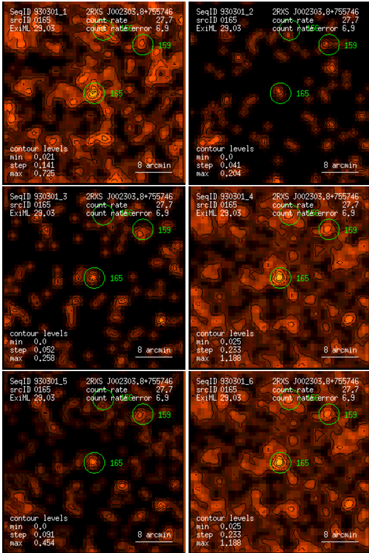
Figure 165: RASS 930301: detection 0165: band rate images, Gaussian filter: (1) PSPC channels 11 – 41, (2) 52 – 90, (3) 91 – 201, (4) 11 – 235, (5) 52 – 201, (6) 11 – 201. Broad band rates in counts/ks. Band rate contour levels in counts/ks/arcmin 2 .
