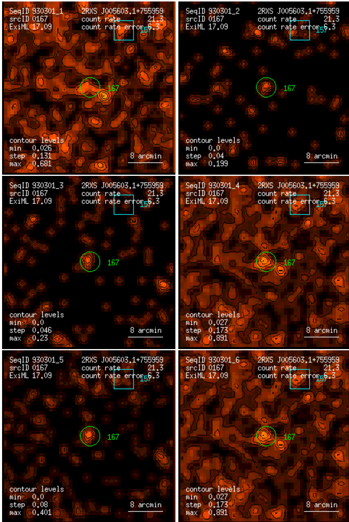
Figure 167: RASS 930301: detection 0167: band rate images, Gaussian filter: (1) PSPC channels 11 – 41, (2) 52 – 90, (3) 91 – 201, (4) 11 – 235, (5) 52 – 201, (6) 11 – 201. Broad band rates in counts/ks. Band rate contour levels in counts/ks/arcmin 2 .
