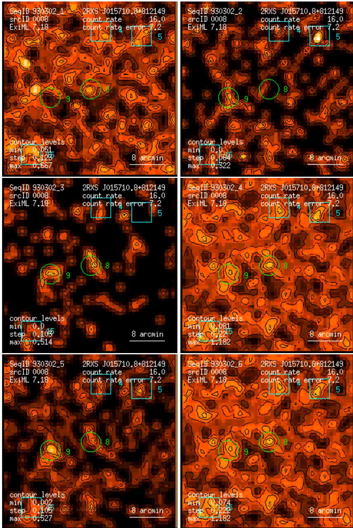
Figure 8: RASS 930302: detection 0008: band rate images, Gaussian filter: (1) PSPC channels 11 – 41, (2) 52 – 90, (3) 91 – 201, (4) 11 – 235, (5) 52 – 201, (6) 11 – 201. Broad band rates in counts/ks. Band rate contour levels in counts/ks/arcmin 2 .
