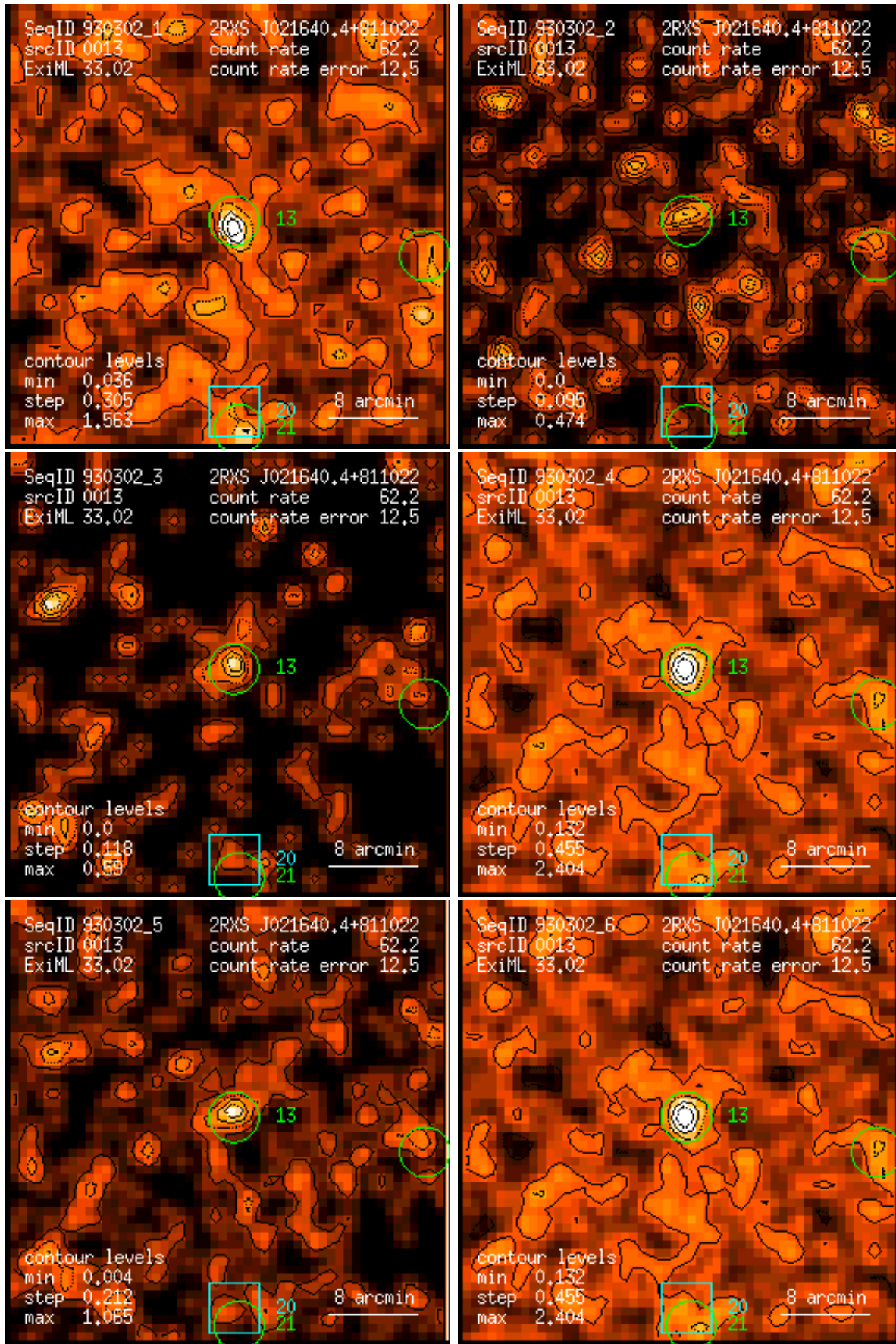
Figure 13: RASS 930302: detection 0013: band rate images, Gaussian filter: (1) PSPC channels 11 – 41, (2) 52 – 90, (3) 91 – 201, (4) 11 – 235, (5) 52 – 201, (6) 11 – 201. Broad band rates in counts/ks. Band rate contour levels in counts/ks/arcmin 2 .
