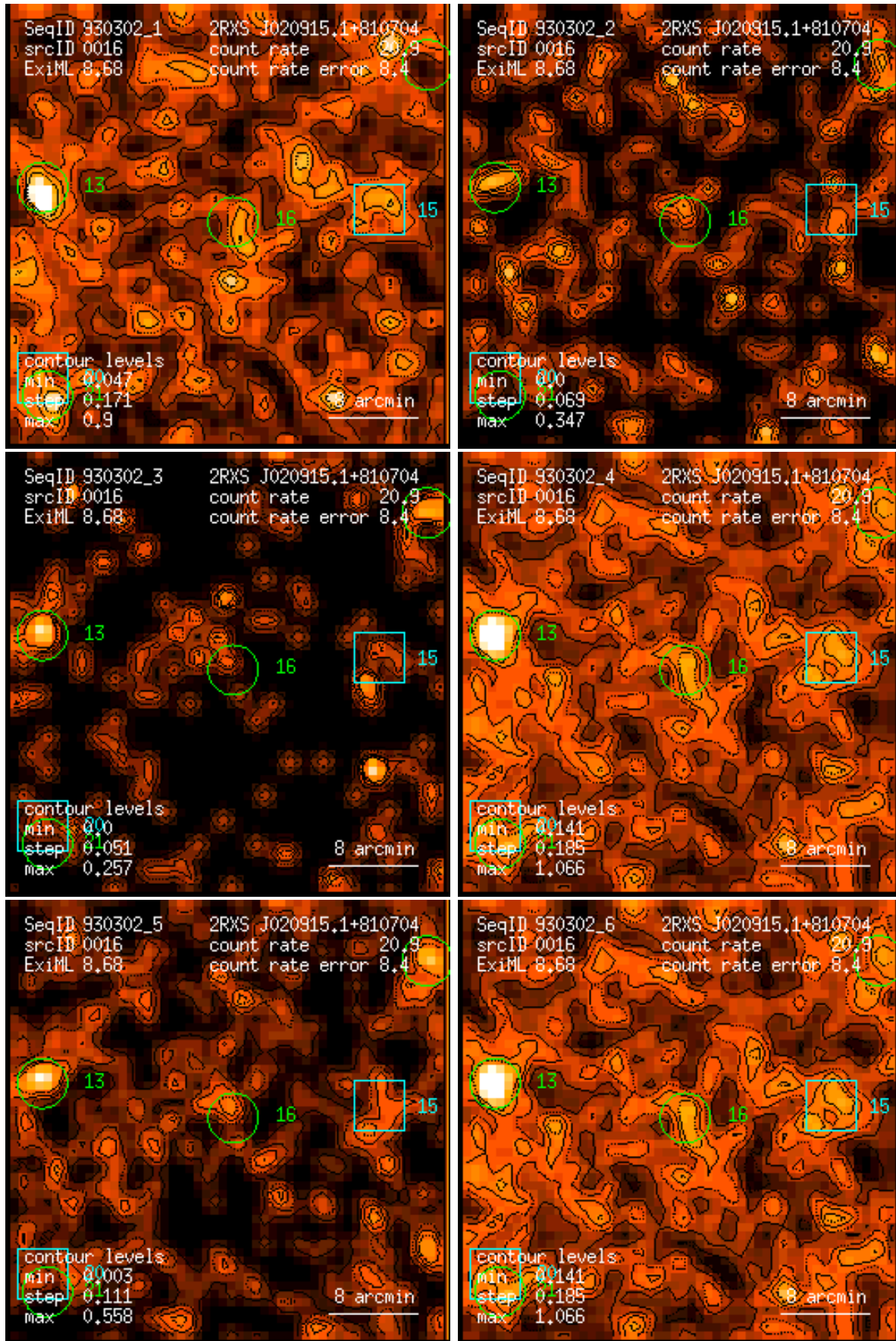
Figure 16: RASS 930302: detection 0016: band rate images, Gaussian filter: (1) PSPC channels 11 – 41, (2) 52 – 90, (3) 91 – 201, (4) 11 – 235, (5) 52 – 201, (6) 11 – 201. Broad band rates in counts/ks. Band rate contour levels in counts/ks/arcmin 2 .
