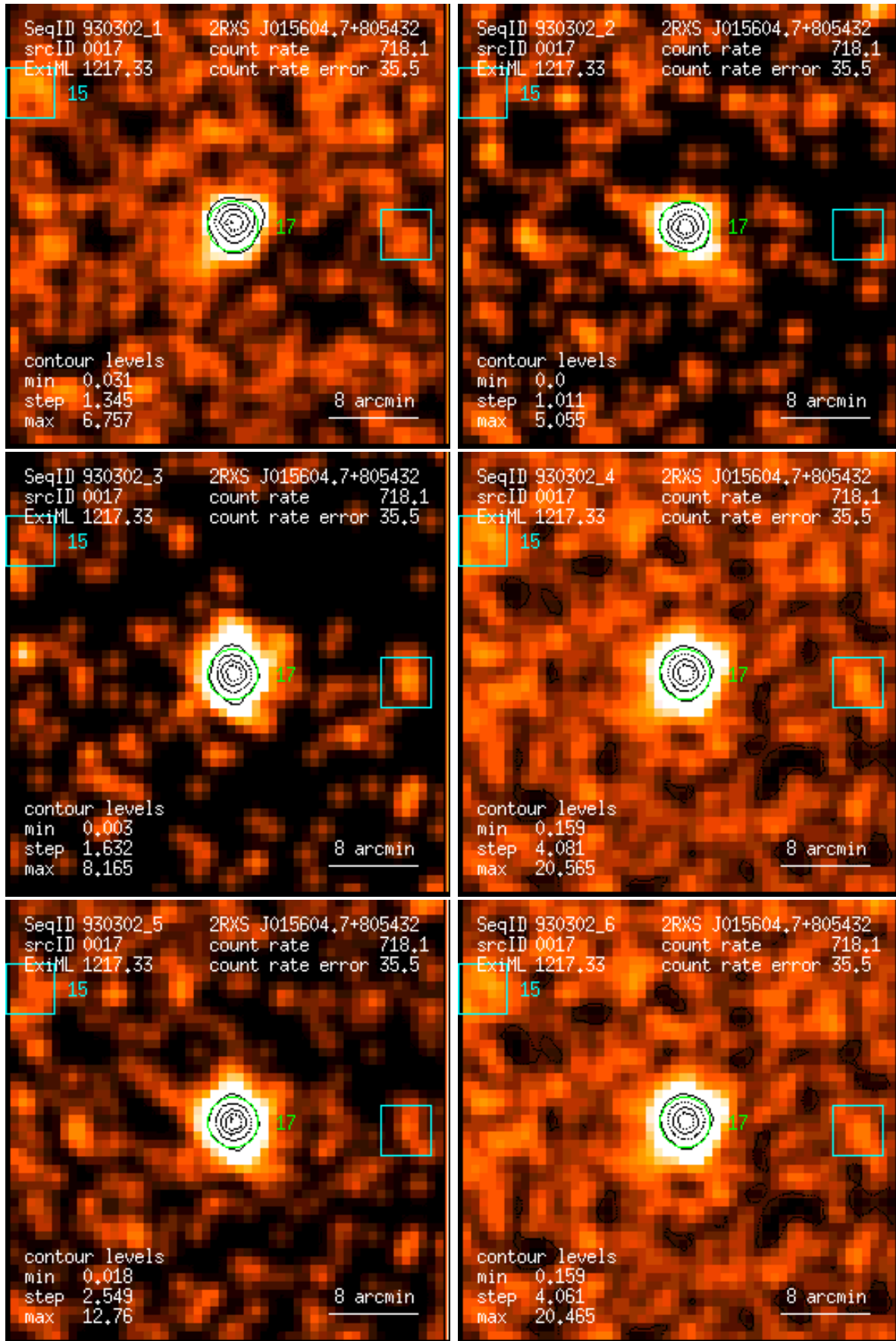
Figure 17: RASS 930302: detection 0017: band rate images, Gaussian filter: (1) PSPC channels 11 – 41, (2) 52 – 90, (3) 91 – 201, (4) 11 – 235, (5) 52 – 201, (6) 11 – 201. Broad band rates in counts/ks. Band rate contour levels in counts/ks/arcmin 2 .
