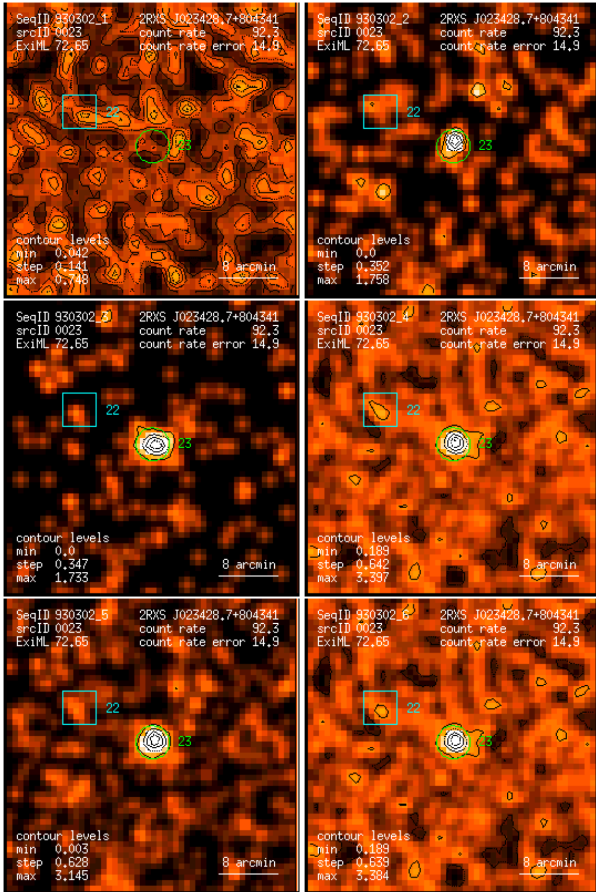
Figure 23: RASS 930302: detection 0023: band rate images, Gaussian filter: (1) PSPC channels 11 – 41, (2) 52 – 90, (3) 91 – 201, (4) 11 – 235, (5) 52 – 201, (6) 11 – 201. Broad band rates in counts/ks. Band rate contour levels in counts/ks/arcmin 2 .
