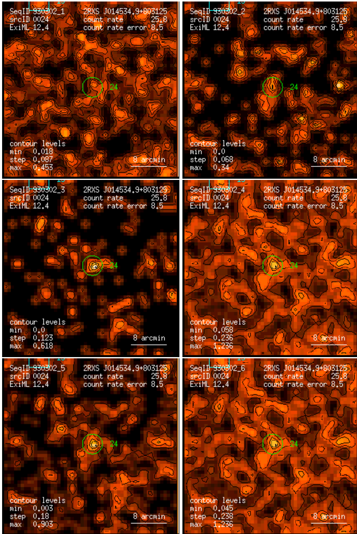
Figure 24: RASS 930302: detection 0024: band rate images, Gaussian filter: (1) PSPC channels 11 – 41, (2) 52 – 90, (3) 91 – 201, (4) 11 – 235, (5) 52 – 201, (6) 11 – 201. Broad band rates in counts/ks. Band rate contour levels in counts/ks/arcmin 2 .
