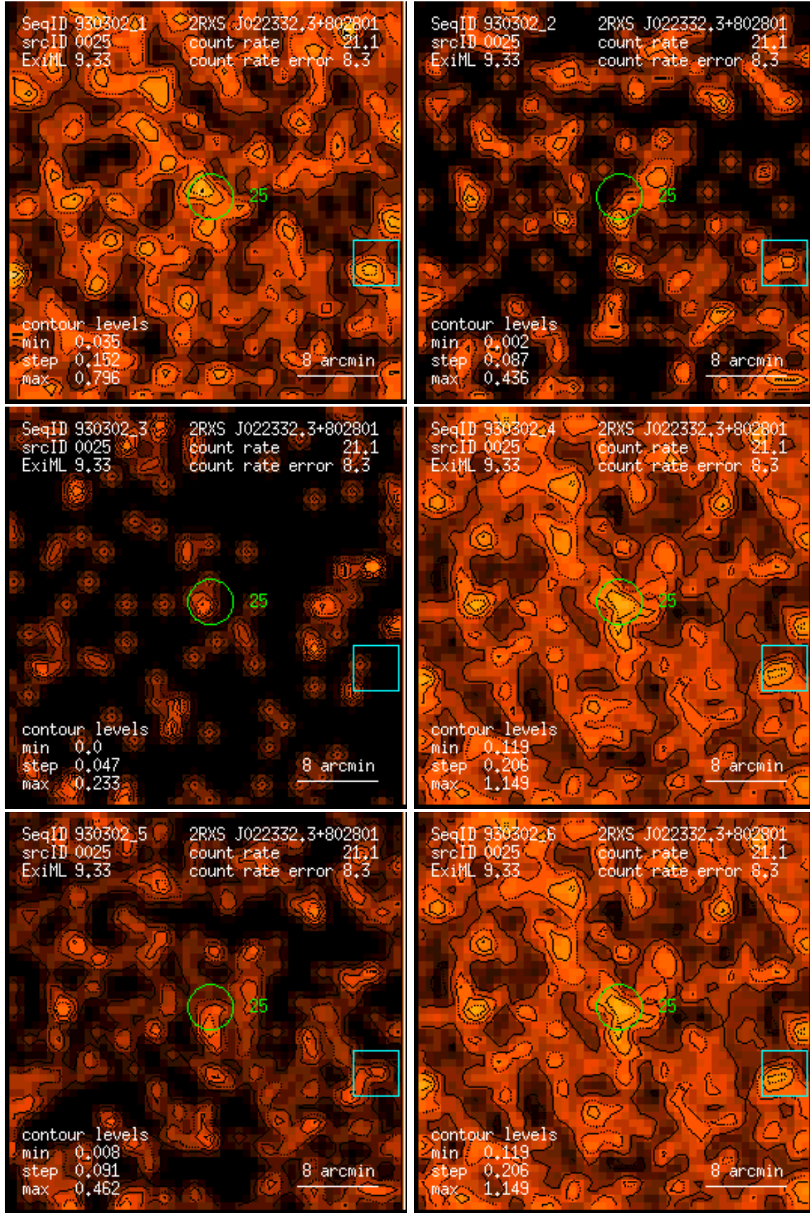
Figure 25: RASS 930302: detection 0025: band rate images, Gaussian filter: (1) PSPC channels 11 – 41, (2) 52 – 90, (3) 91 – 201, (4) 11 – 235, (5) 52 – 201, (6) 11 – 201. Broad band rates in counts/ks. Band rate contour levels in counts/ks/arcmin 2 .
