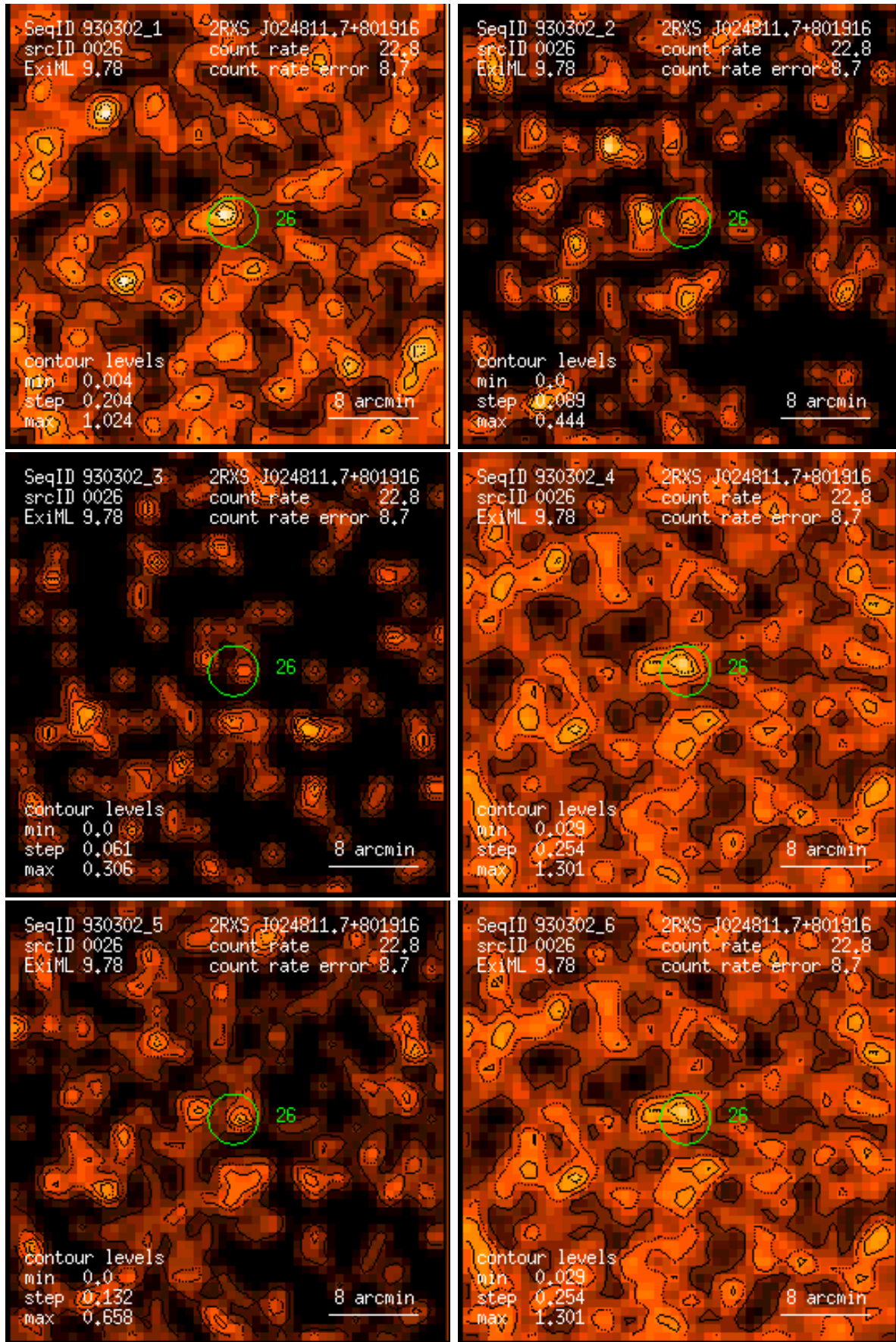
Figure 26: RASS 930302: detection 0026: band rate images, Gaussian filter: (1) PSPC channels 11 – 41, (2) 52 – 90, (3) 91 – 201, (4) 11 – 235, (5) 52 – 201, (6) 11 – 201. Broad band rates in counts/ks. Band rate contour levels in counts/ks/arcmin 2 .
