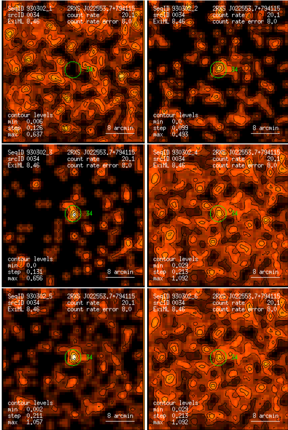
Figure 34: RASS 930302: detection 0034: band rate images, Gaussian filter: (1) PSPC channels 11 – 41, (2) 52 – 90, (3) 91 – 201, (4) 11 – 235, (5) 52 – 201, (6) 11 – 201. Broad band rates in counts/ks. Band rate contour levels in counts/ks/arcmin 2 .
