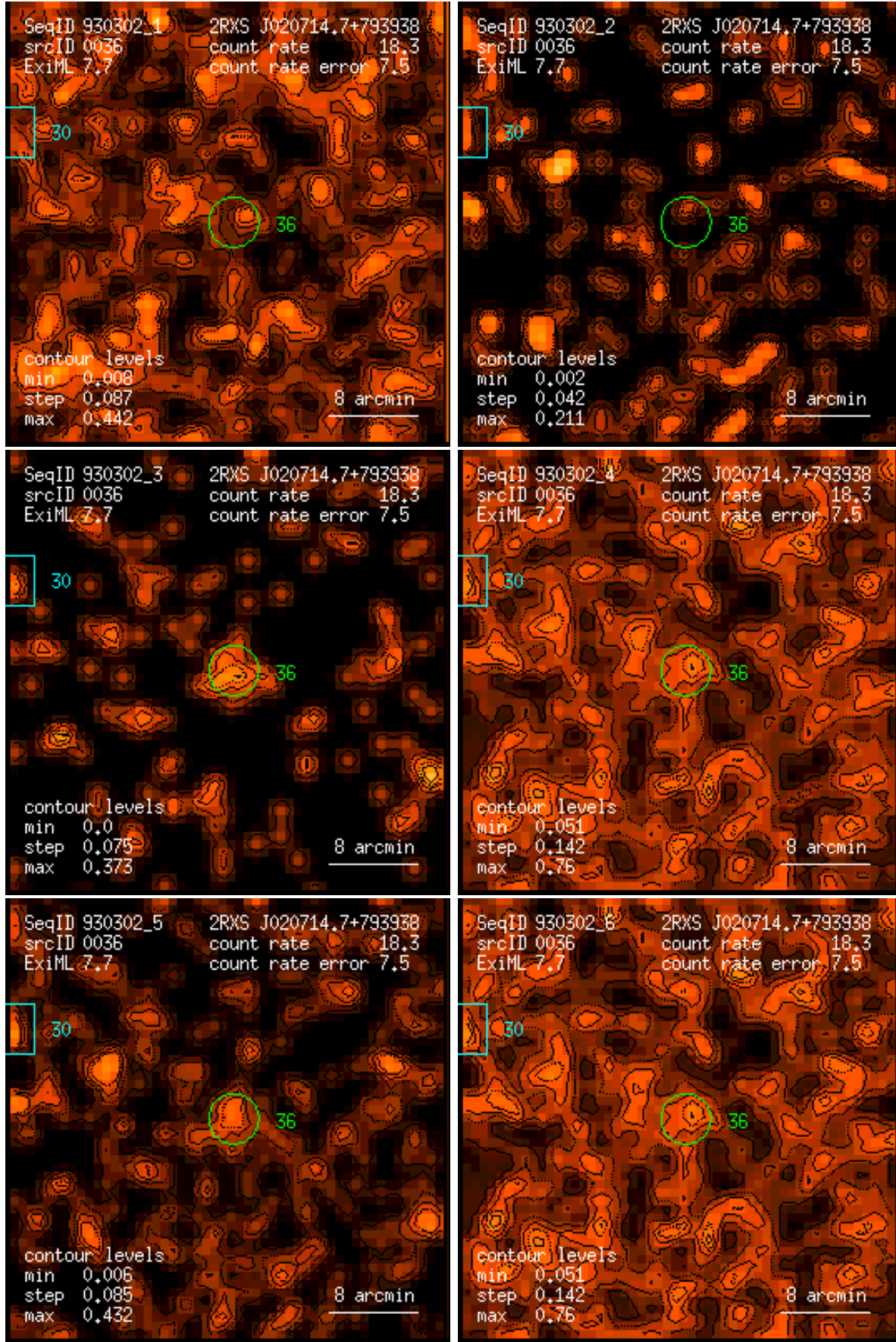
Figure 36: RASS 930302: detection 0036: band rate images, Gaussian filter: (1) PSPC channels 11 – 41, (2) 52 – 90, (3) 91 – 201, (4) 11 – 235, (5) 52 – 201, (6) 11 – 201. Broad band rates in counts/ks. Band rate contour levels in counts/ks/arcmin 2 .
