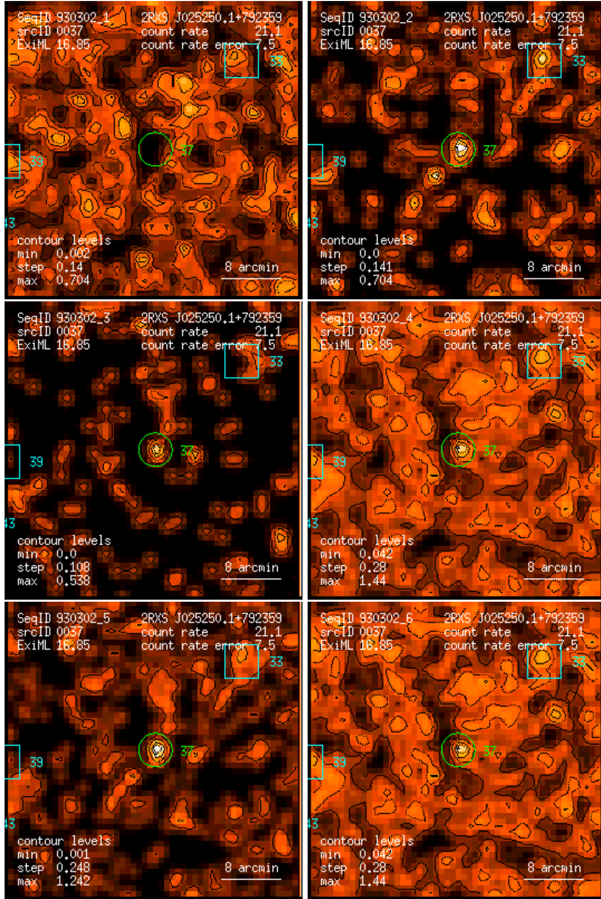
Figure 37: RASS 930302: detection 0037: band rate images, Gaussian filter: (1) PSPC channels 11 – 41, (2) 52 – 90, (3) 91 – 201, (4) 11 – 235, (5) 52 – 201, (6) 11 – 201. Broad band rates in counts/ks. Band rate contour levels in counts/ks/arcmin 2 .
