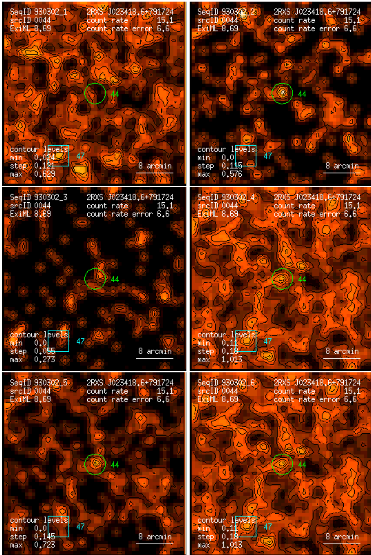
Figure 44: RASS 930302: detection 0044: band rate images, Gaussian filter: (1) PSPC channels 11 – 41, (2) 52 – 90, (3) 91 – 201, (4) 11 – 235, (5) 52 – 201, (6) 11 – 201. Broad band rates in counts/ks. Band rate contour levels in counts/ks/arcmin 2 .
