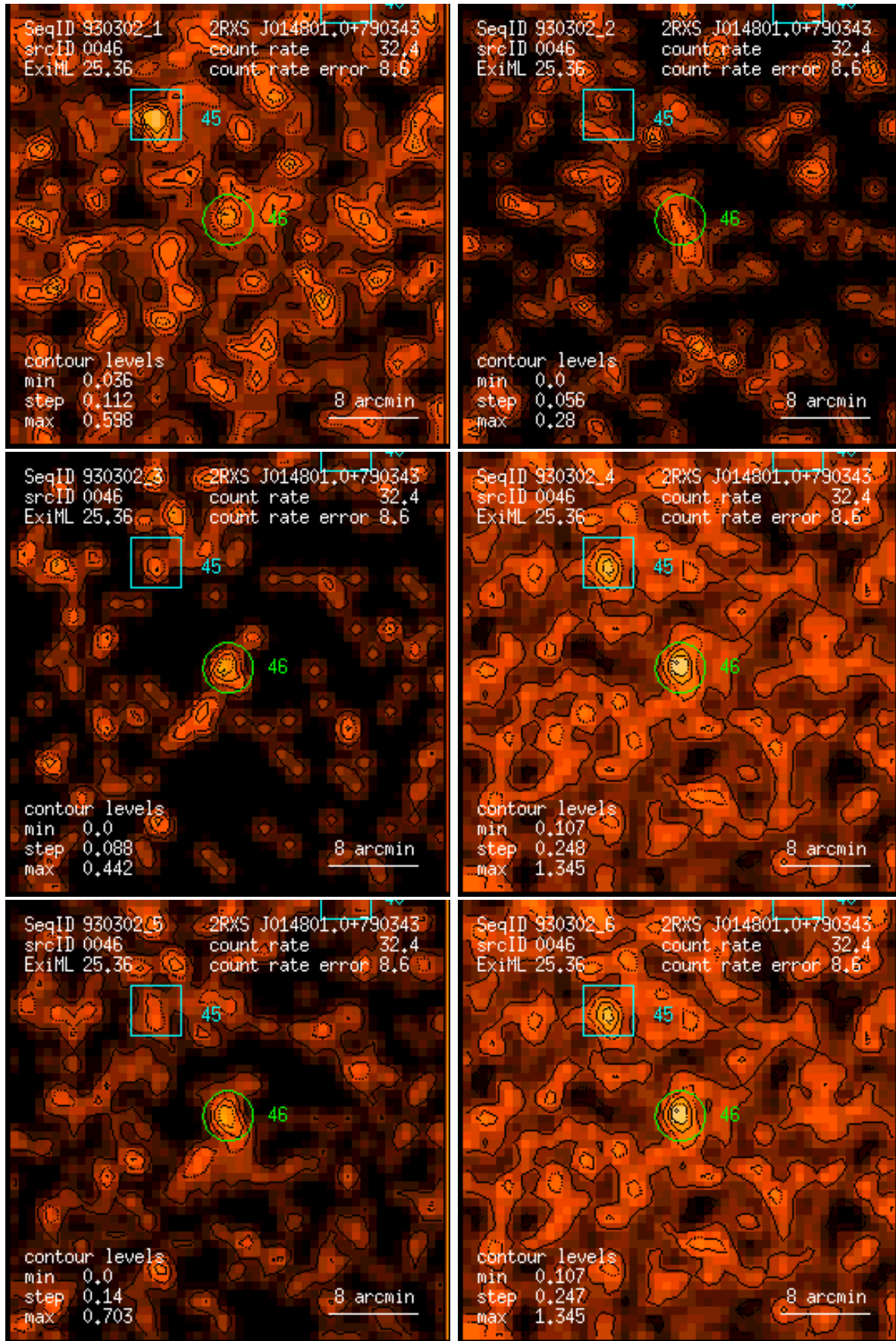
Figure 46: RASS 930302: detection 0046: band rate images, Gaussian filter: (1) PSPC channels 11 – 41, (2) 52 – 90, (3) 91 – 201, (4) 11 – 235, (5) 52 – 201, (6) 11 – 201. Broad band rates in counts/ks. Band rate contour levels in counts/ks/arcmin 2 .
