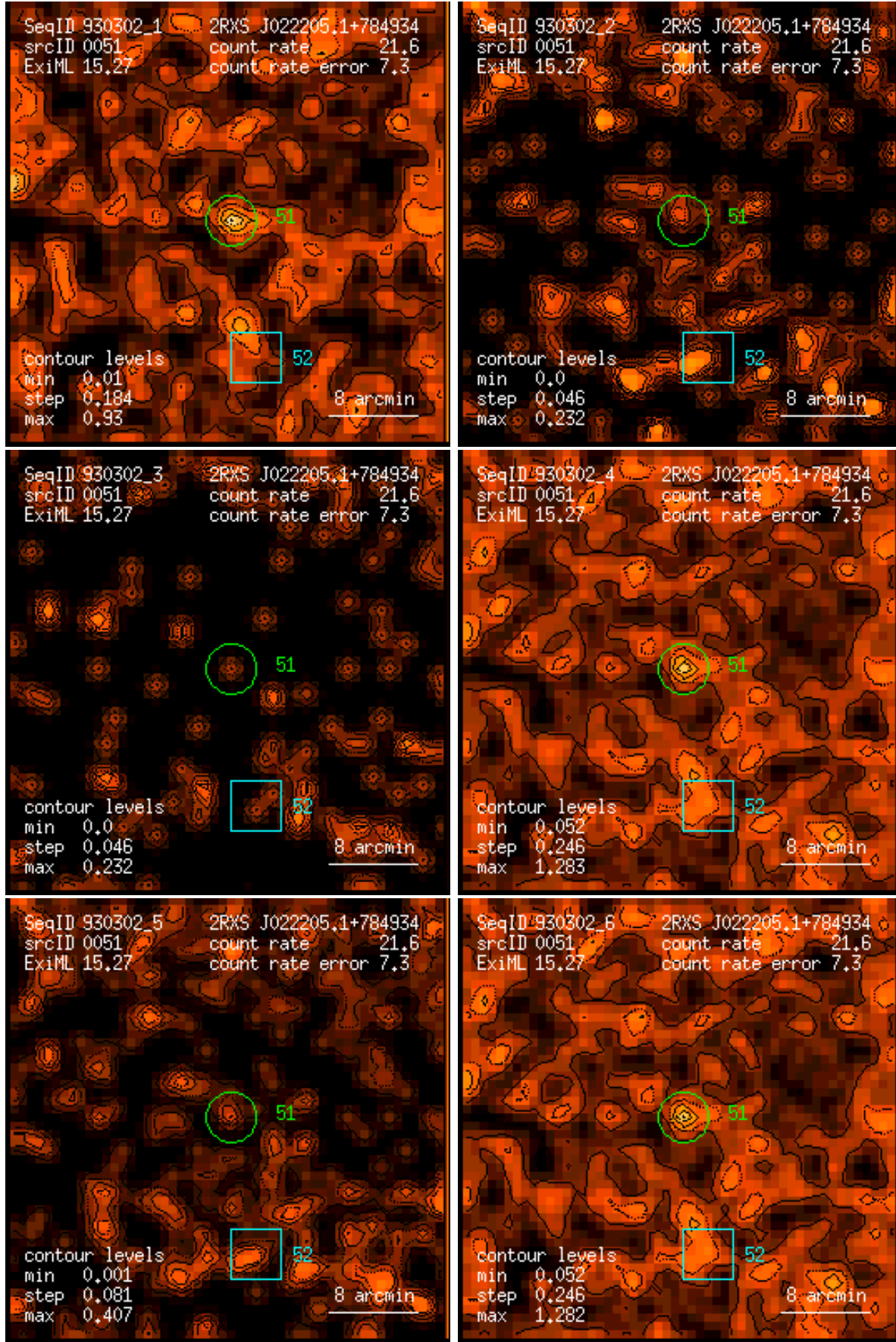
Figure 51: RASS 930302: detection 0051: band rate images, Gaussian filter: (1) PSPC channels 11 – 41, (2) 52 – 90, (3) 91 – 201, (4) 11 – 235, (5) 52 – 201, (6) 11 – 201. Broad band rates in counts/ks. Band rate contour levels in counts/ks/arcmin 2 .
