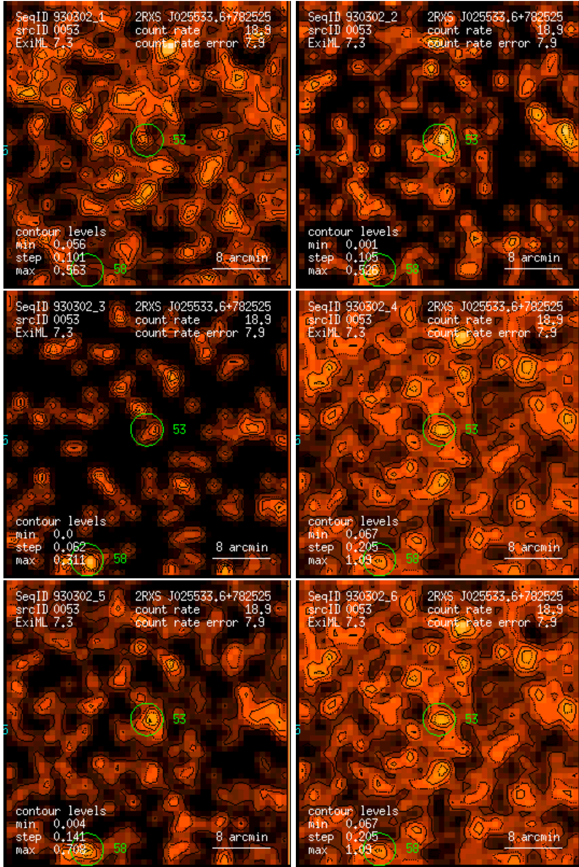
Figure 53: RASS 930302: detection 0053: band rate images, Gaussian filter: (1) PSPC channels 11 – 41, (2) 52 – 90, (3) 91 – 201, (4) 11 – 235, (5) 52 – 201, (6) 11 – 201. Broad band rates in counts/ks. Band rate contour levels in counts/ks/arcmin 2 .
